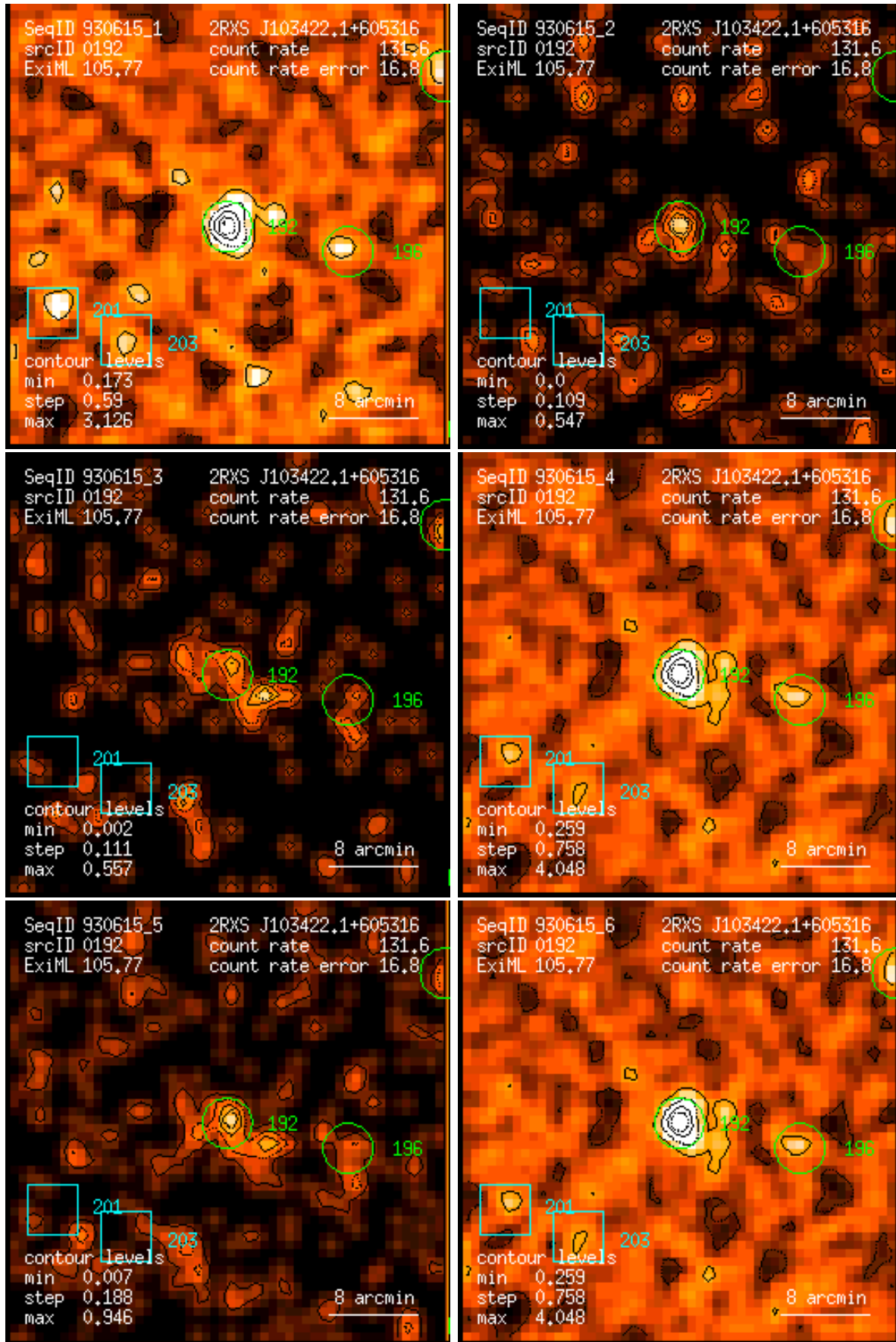
Figure 192: RASS 930615: detection 0192: band rate images, Gaussian filter: (1) PSPC channels 11 – 41, (2) 52 – 90, (3) 91 – 201, (4) 11 – 235, (5) 52 – 201, (6) 11 – 201. Broad band rates in counts/ks. Band rate contour levels in counts/ks/arcmin 2 .
