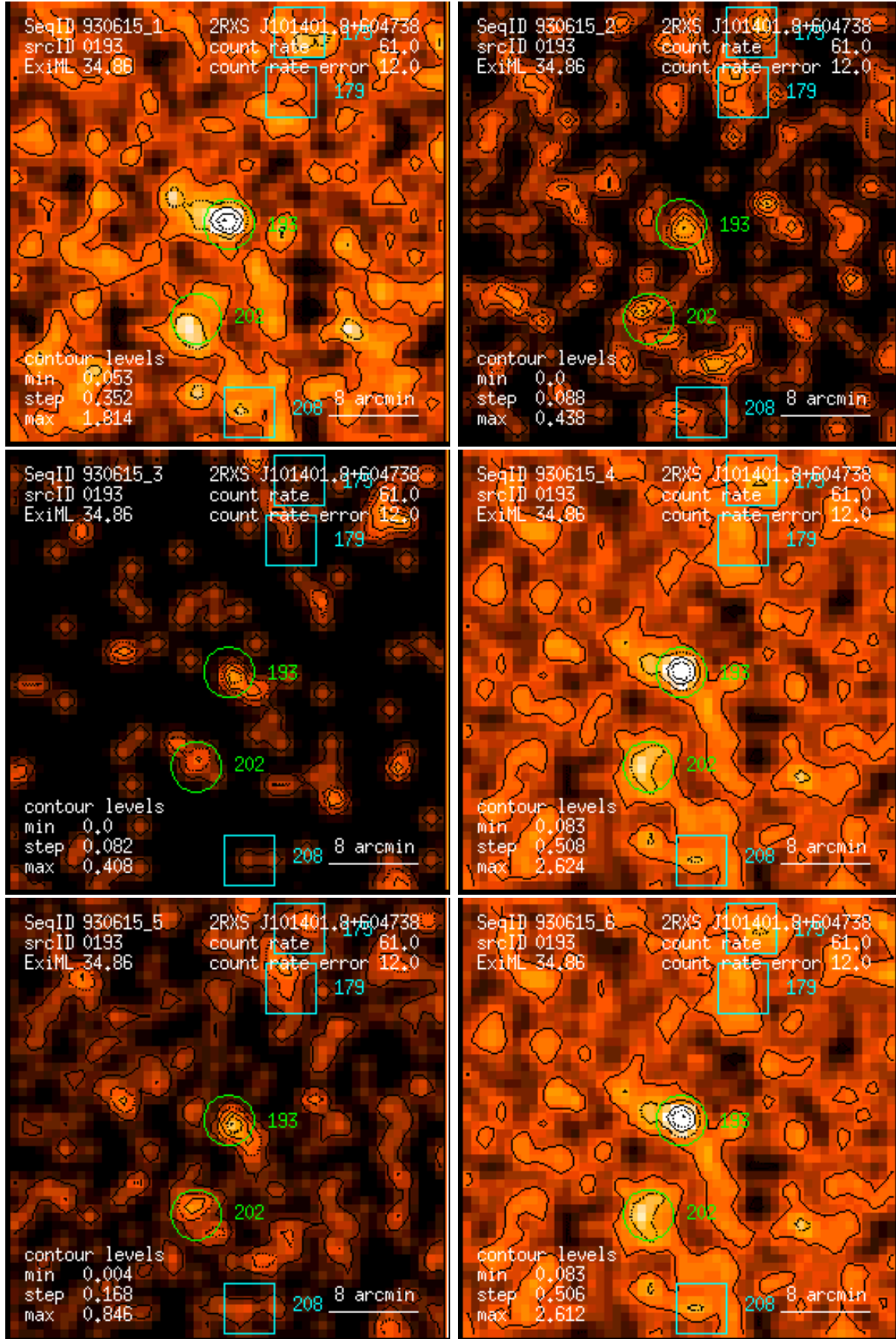
Figure 193: RASS 930615: detection 0193: band rate images, Gaussian filter: (1) PSPC channels 11 – 41, (2) 52 – 90, (3) 91 – 201, (4) 11 – 235, (5) 52 – 201, (6) 11 – 201. Broad band rates in counts/ks. Band rate contour levels in counts/ks/arcmin 2 .
