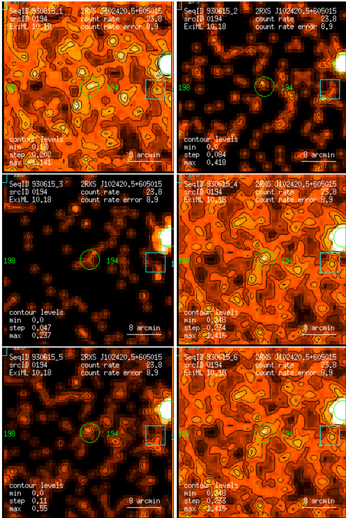
Figure 194: RASS 930615: detection 0194: band rate images, Gaussian filter: (1) PSPC channels 11 – 41, (2) 52 – 90, (3) 91 – 201, (4) 11 – 235, (5) 52 – 201, (6) 11 – 201. Broad band rates in counts/ks. Band rate contour levels in counts/ks/arcmin 2 .
