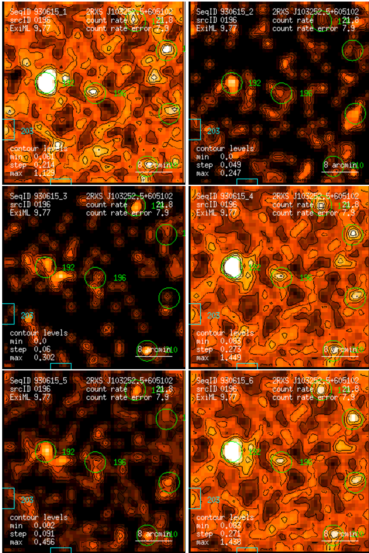
Figure 196: RASS 930615: detection 0196: band rate images, Gaussian filter: (1) PSPC channels 11 – 41, (2) 52 – 90, (3) 91 – 201, (4) 11 – 235, (5) 52 – 201, (6) 11 – 201. Broad band rates in counts/ks. Band rate contour levels in counts/ks/arcmin 2 .
