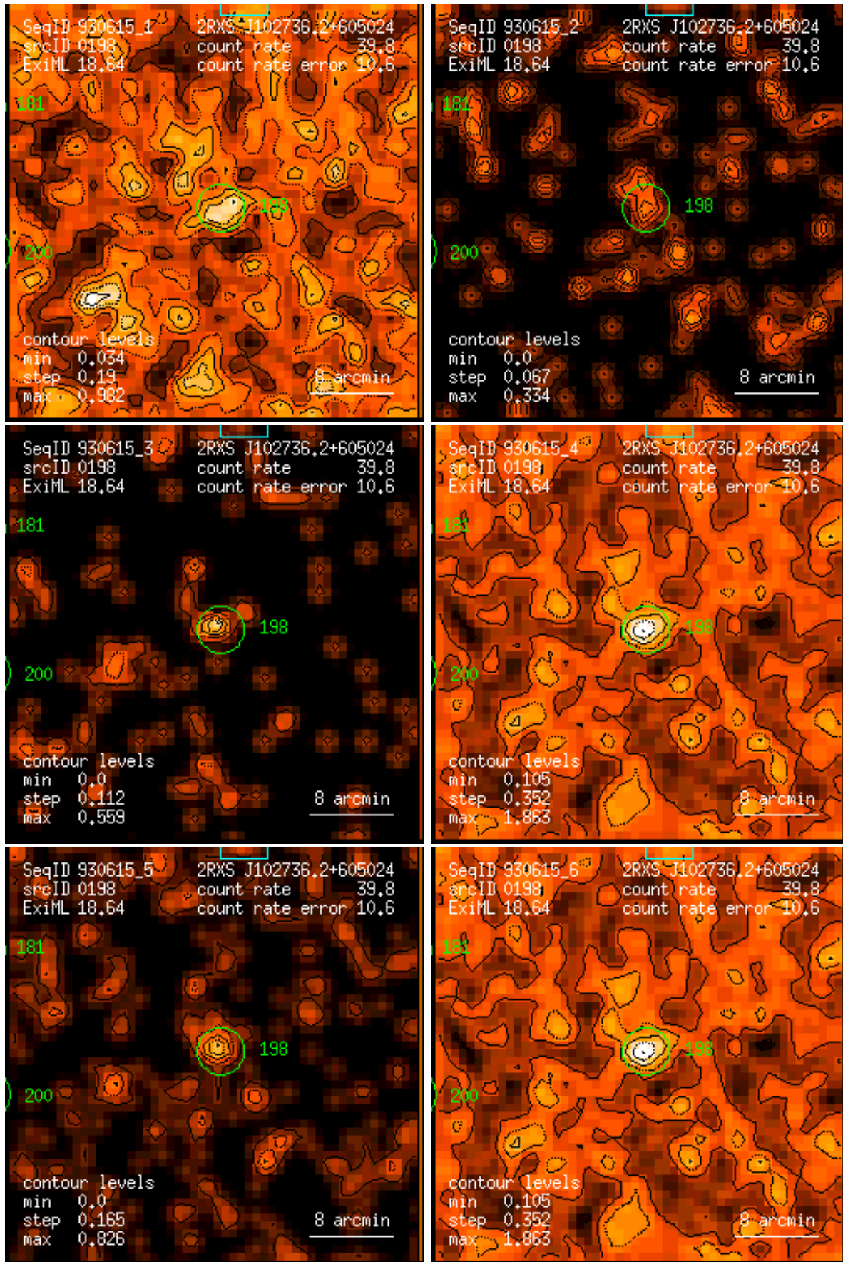
Figure 198: RASS 930615: detection 0198: band rate images, Gaussian filter: (1) PSPC channels 11 – 41, (2) 52 – 90, (3) 91 – 201, (4) 11 – 235, (5) 52 – 201, (6) 11 – 201. Broad band rates in counts/ks. Band rate contour levels in counts/ks/arcmin 2 .
