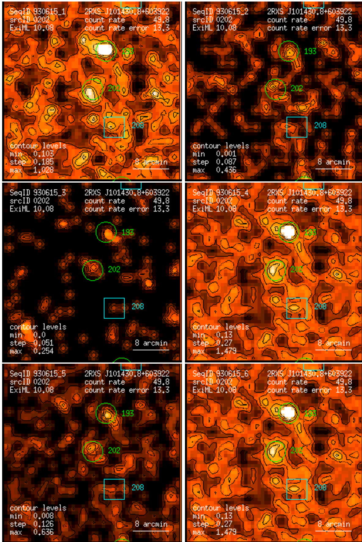
Figure 202: RASS 930615: detection 0202: band rate images, Gaussian filter: (1) PSPC channels 11 – 41, (2) 52 – 90, (3) 91 – 201, (4) 11 – 235, (5) 52 – 201, (6) 11 – 201. Broad band rates in counts/ks. Band rate contour levels in counts/ks/arcmin 2 .
