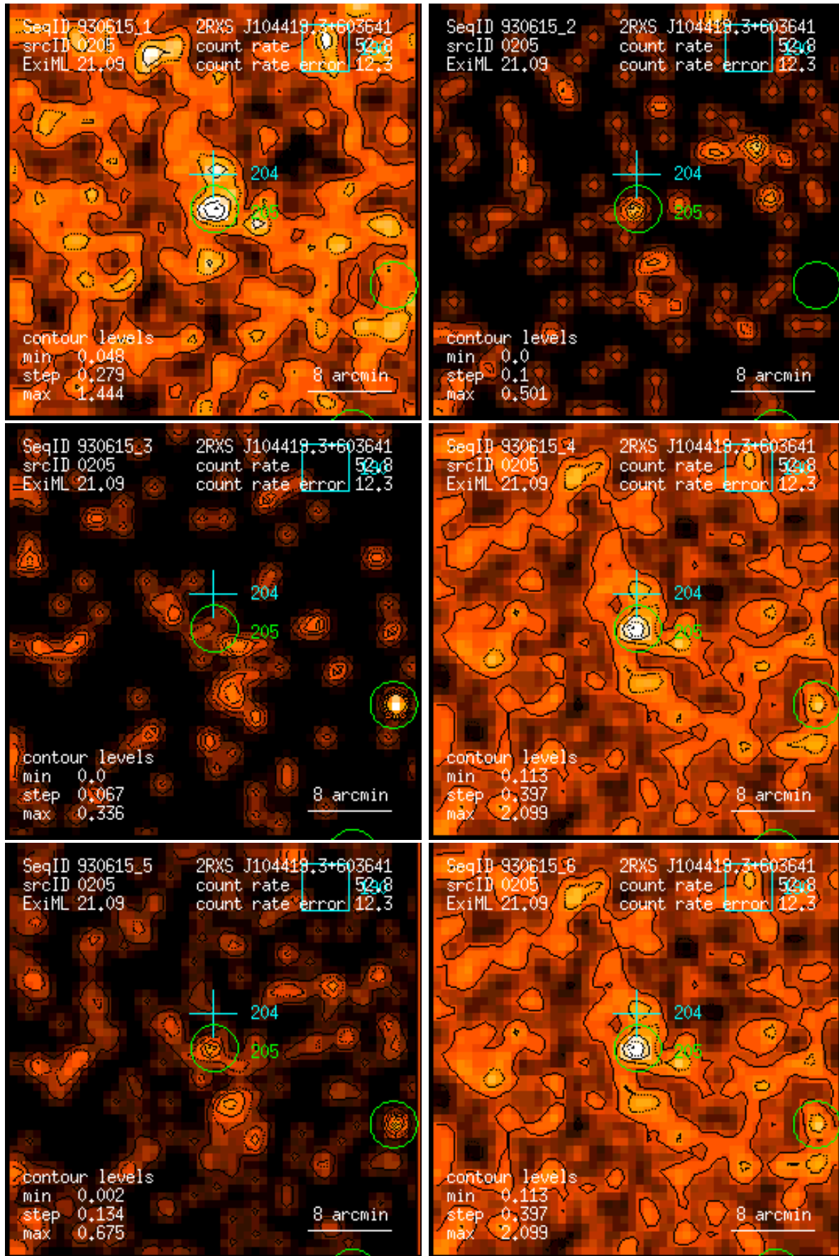
Figure 205: RASS 930615: detection 0205: band rate images, Gaussian filter: (1) PSPC channels 11 – 41, (2) 52 – 90, (3) 91 – 201, (4) 11 – 235, (5) 52 – 201, (6) 11 – 201. Broad band rates in counts/ks. Band rate contour levels in counts/ks/arcmin 2 .
