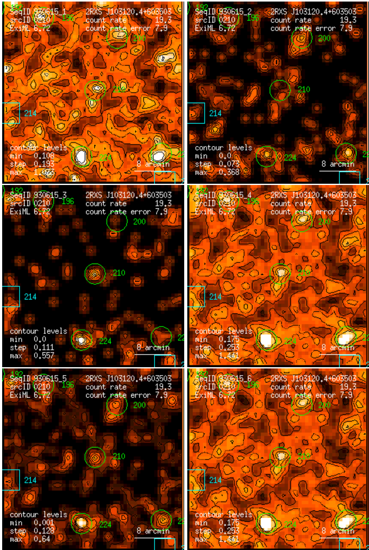
Figure 210: RASS 930615: detection 0210: band rate images, Gaussian filter: (1) PSPC channels 11 – 41, (2) 52 – 90, (3) 91 – 201, (4) 11 – 235, (5) 52 – 201, (6) 11 – 201. Broad band rates in counts/ks. Band rate contour levels in counts/ks/arcmin 2 .
