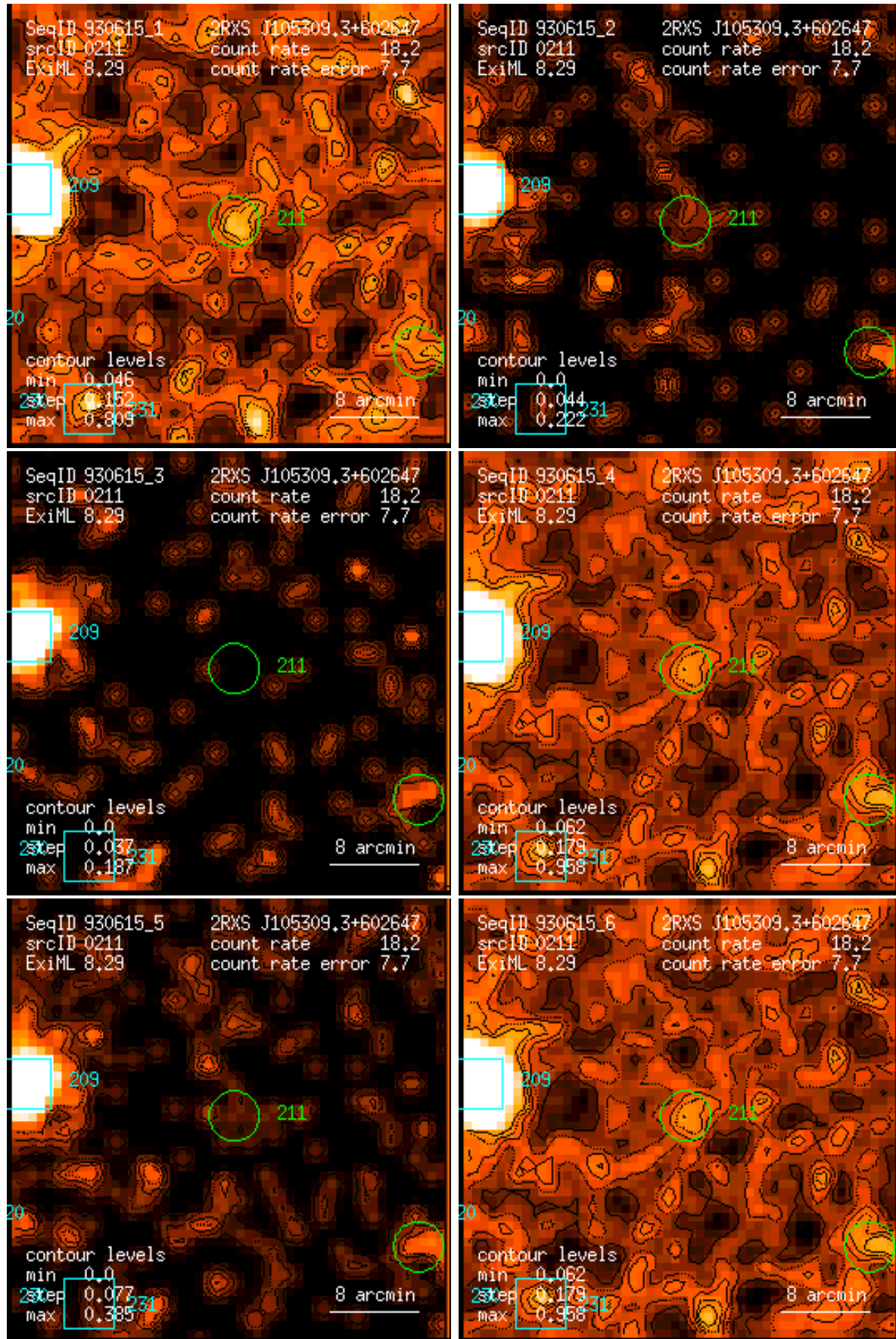
Figure 211: RASS 930615: detection 0211: band rate images, Gaussian filter: (1) PSPC channels 11 – 41, (2) 52 – 90, (3) 91 – 201, (4) 11 – 235, (5) 52 – 201, (6) 11 – 201. Broad band rates in counts/ks. Band rate contour levels in counts/ks/arcmin 2 .
