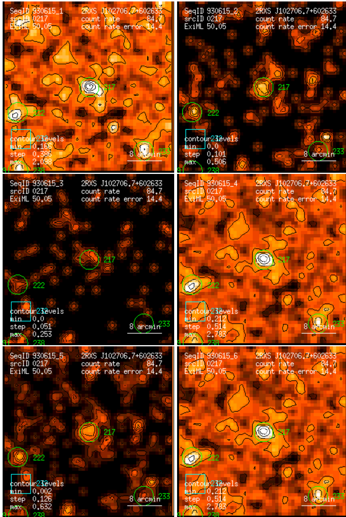
Figure 217: RASS 930615: detection 0217: band rate images, Gaussian filter: (1) PSPC channels 11 – 41, (2) 52 – 90, (3) 91 – 201, (4) 11 – 235, (5) 52 – 201, (6) 11 – 201. Broad band rates in counts/ks. Band rate contour levels in counts/ks/arcmin 2 .
