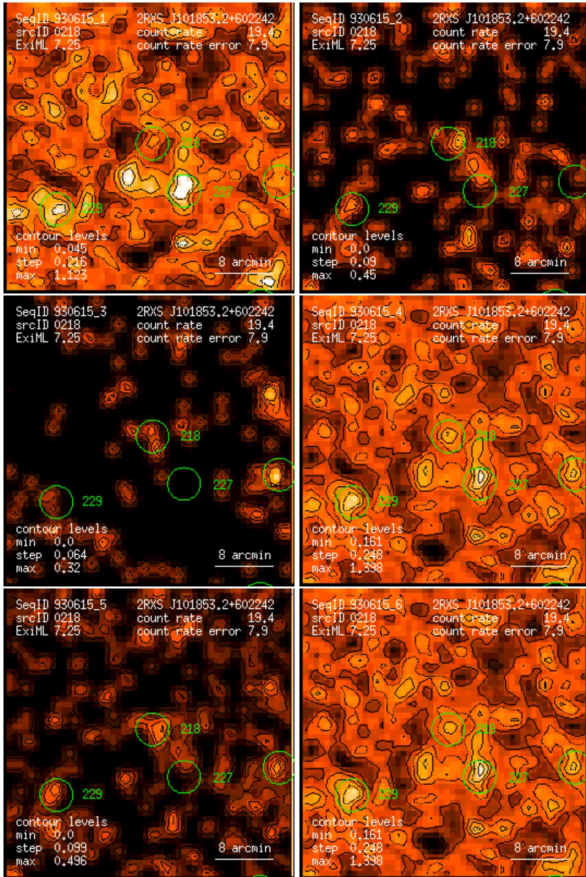
Figure 218: RASS 930615: detection 0218: band rate images, Gaussian filter: (1) PSPC channels 11 – 41, (2) 52 – 90, (3) 91 – 201, (4) 11 – 235, (5) 52 – 201, (6) 11 – 201. Broad band rates in counts/ks. Band rate contour levels in counts/ks/arcmin 2 .
