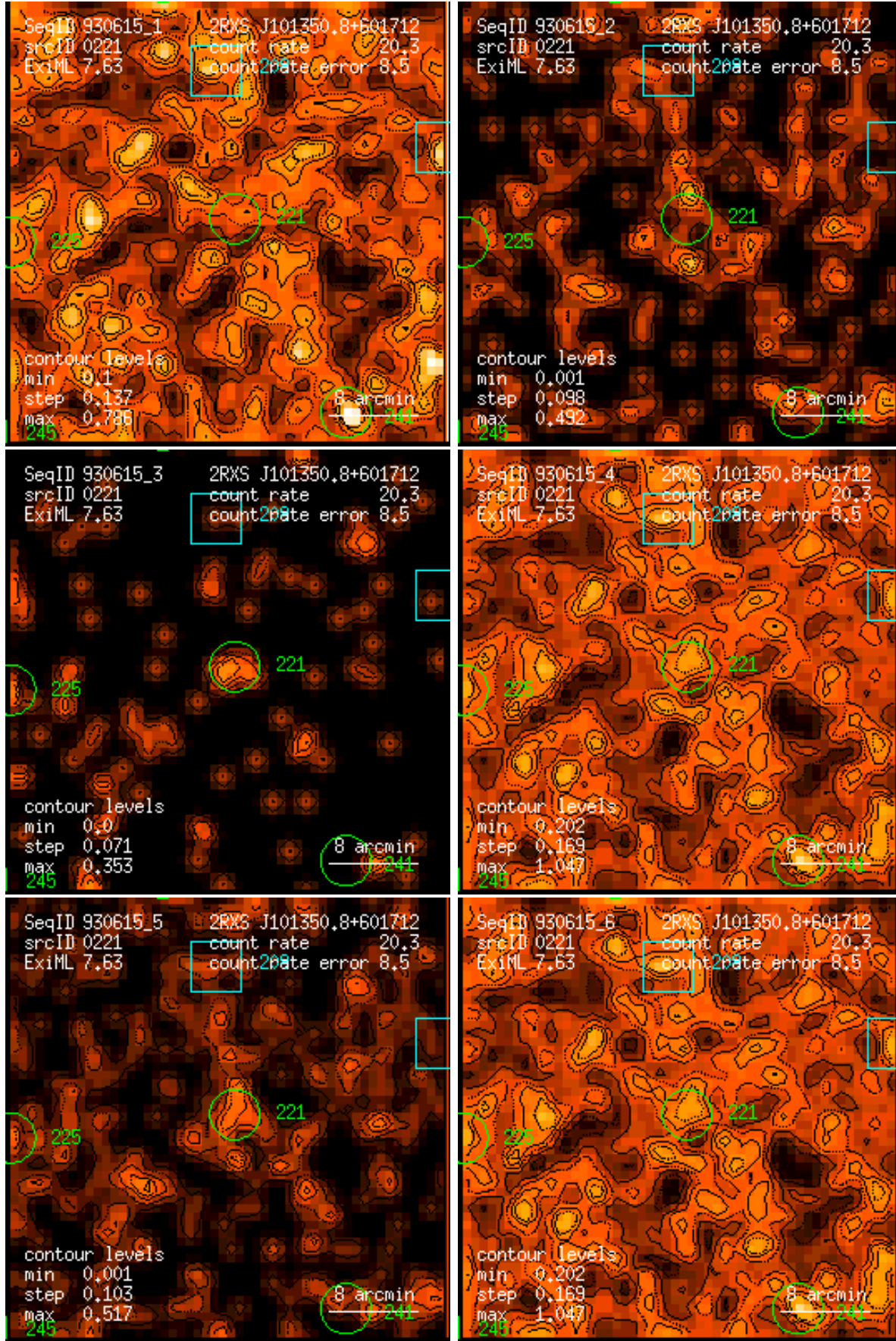
Figure 221: RASS 930615: detection 0221: band rate images, Gaussian filter: (1) PSPC channels 11 – 41, (2) 52 – 90, (3) 91 – 201, (4) 11 – 235, (5) 52 – 201, (6) 11 – 201. Broad band rates in counts/ks. Band rate contour levels in counts/ks/arcmin 2 .
