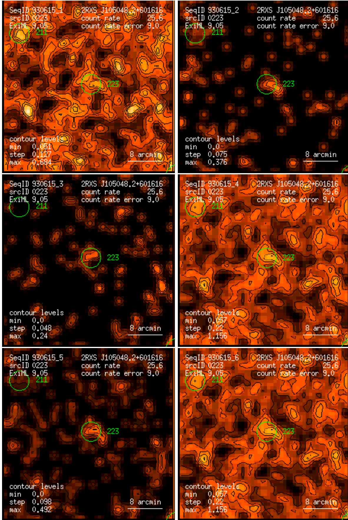
Figure 223: RASS 930615: detection 0223: band rate images, Gaussian filter: (1) PSPC channels 11 – 41, (2) 52 – 90, (3) 91 – 201, (4) 11 – 235, (5) 52 – 201, (6) 11 – 201. Broad band rates in counts/ks. Band rate contour levels in counts/ks/arcmin 2 .
