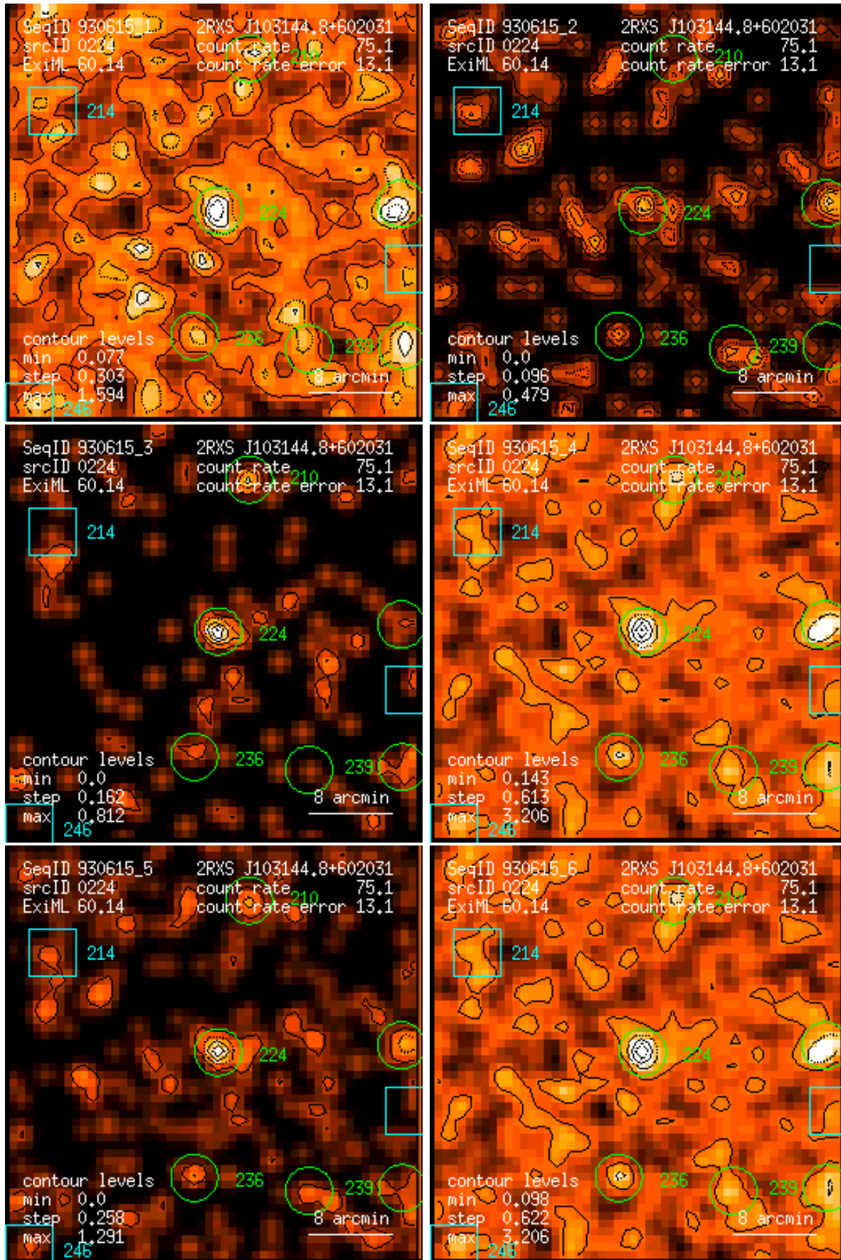
Figure 224: RASS 930615: detection 0224: band rate images, Gaussian filter: (1) PSPC channels 11 – 41, (2) 52 – 90, (3) 91 – 201, (4) 11 – 235, (5) 52 – 201, (6) 11 – 201. Broad band rates in counts/ks. Band rate contour levels in counts/ks/arcmin 2 .
