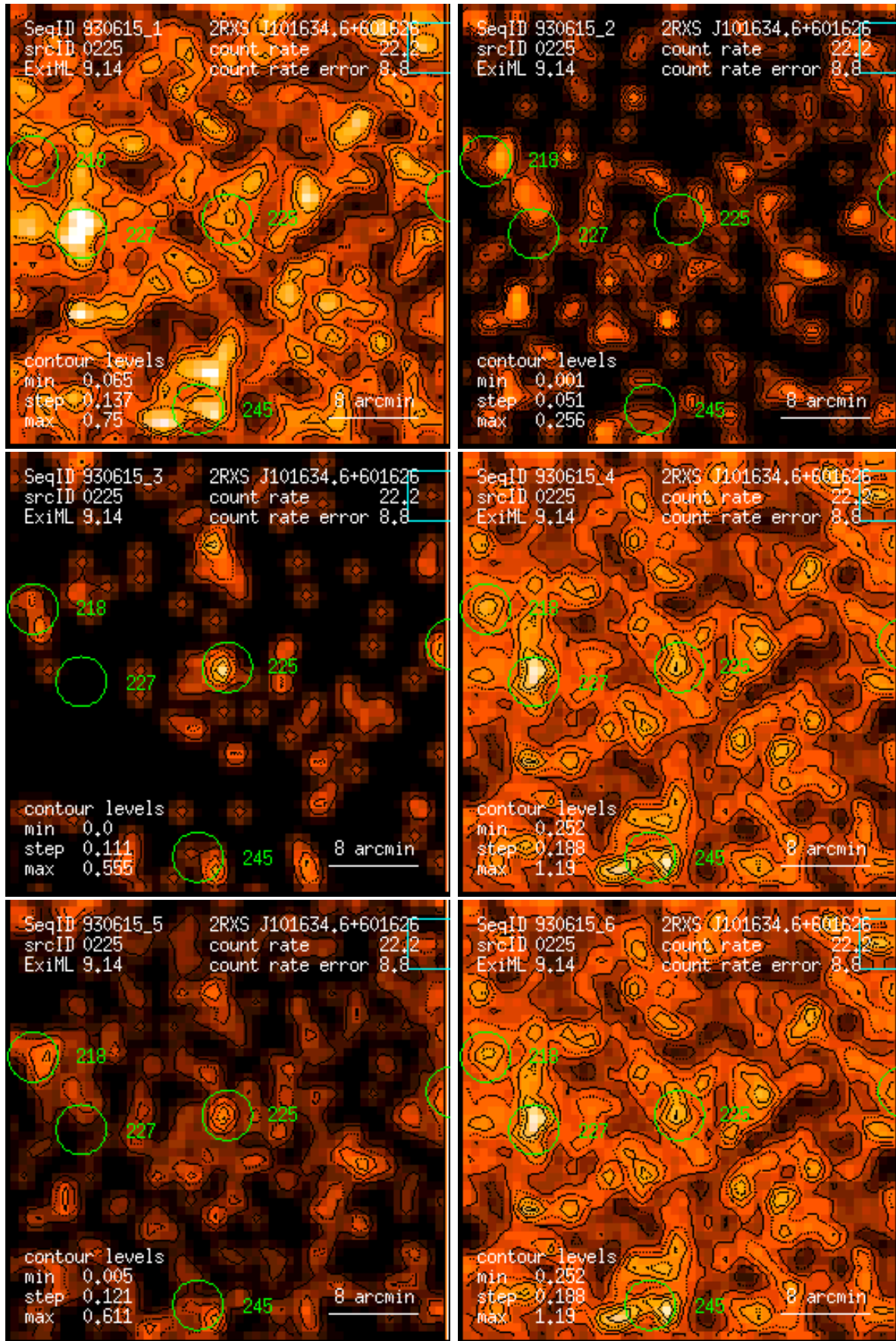
Figure 225: RASS 930615: detection 0225: band rate images, Gaussian filter: (1) PSPC channels 11 – 41, (2) 52 – 90, (3) 91 – 201, (4) 11 – 235, (5) 52 – 201, (6) 11 – 201. Broad band rates in counts/ks. Band rate contour levels in counts/ks/arcmin 2 .
