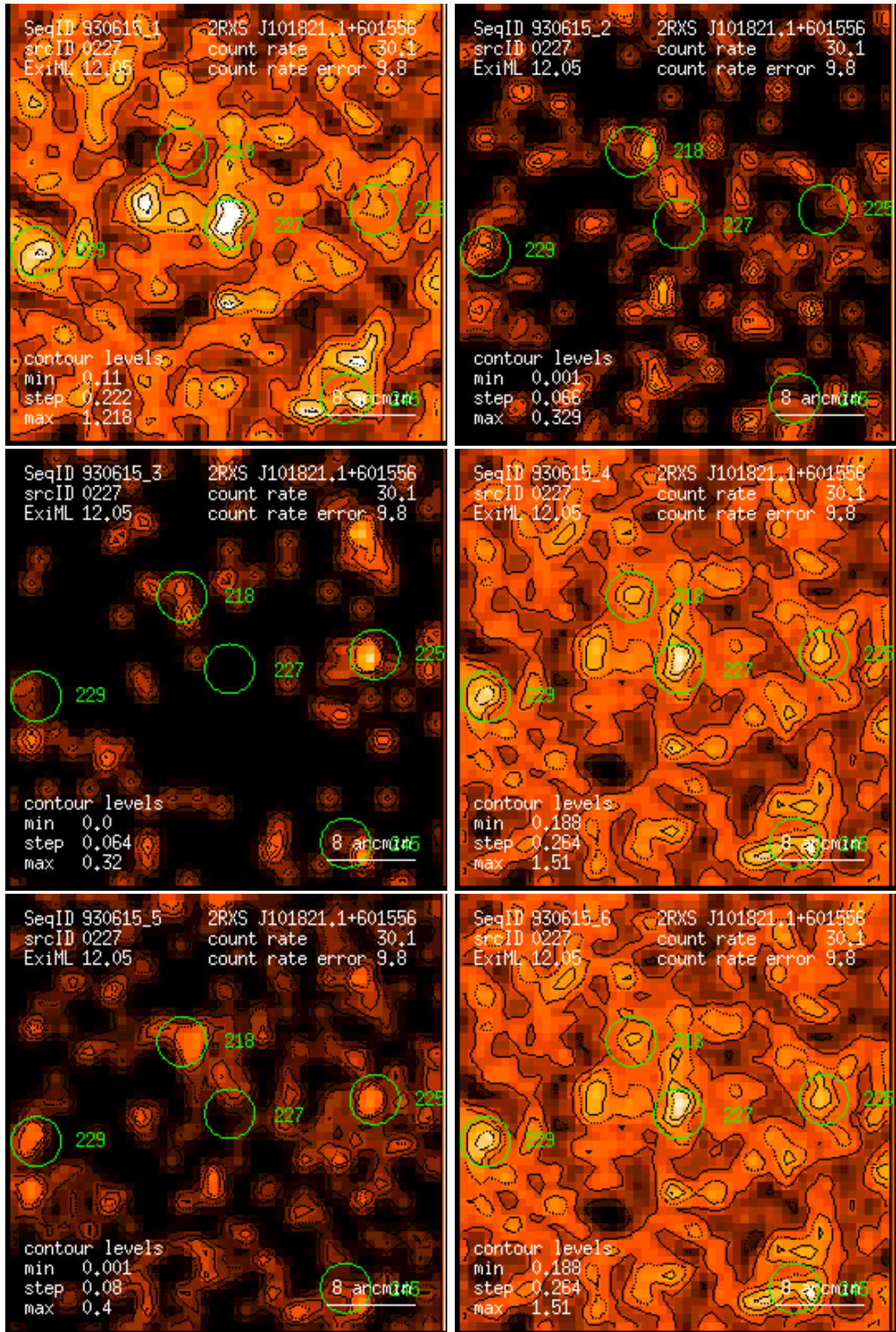
Figure 227: RASS 930615: detection 0227: band rate images, Gaussian filter: (1) PSPC channels 11 – 41, (2) 52 – 90, (3) 91 – 201, (4) 11 – 235, (5) 52 – 201, (6) 11 – 201. Broad band rates in counts/ks. Band rate contour levels in counts/ks/arcmin 2 .
