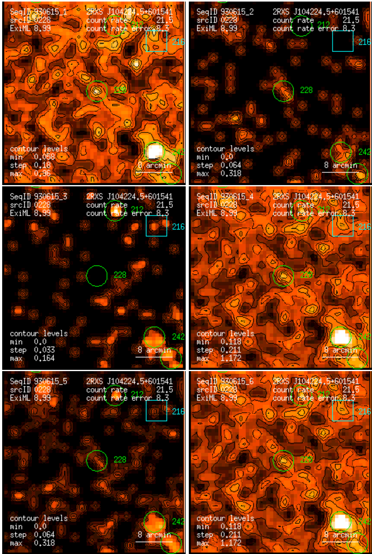
Figure 228: RASS 930615: detection 0228: band rate images, Gaussian filter: (1) PSPC channels 11 – 41, (2) 52 – 90, (3) 91 – 201, (4) 11 – 235, (5) 52 – 201, (6) 11 – 201. Broad band rates in counts/ks. Band rate contour levels in counts/ks/arcmin 2 .
