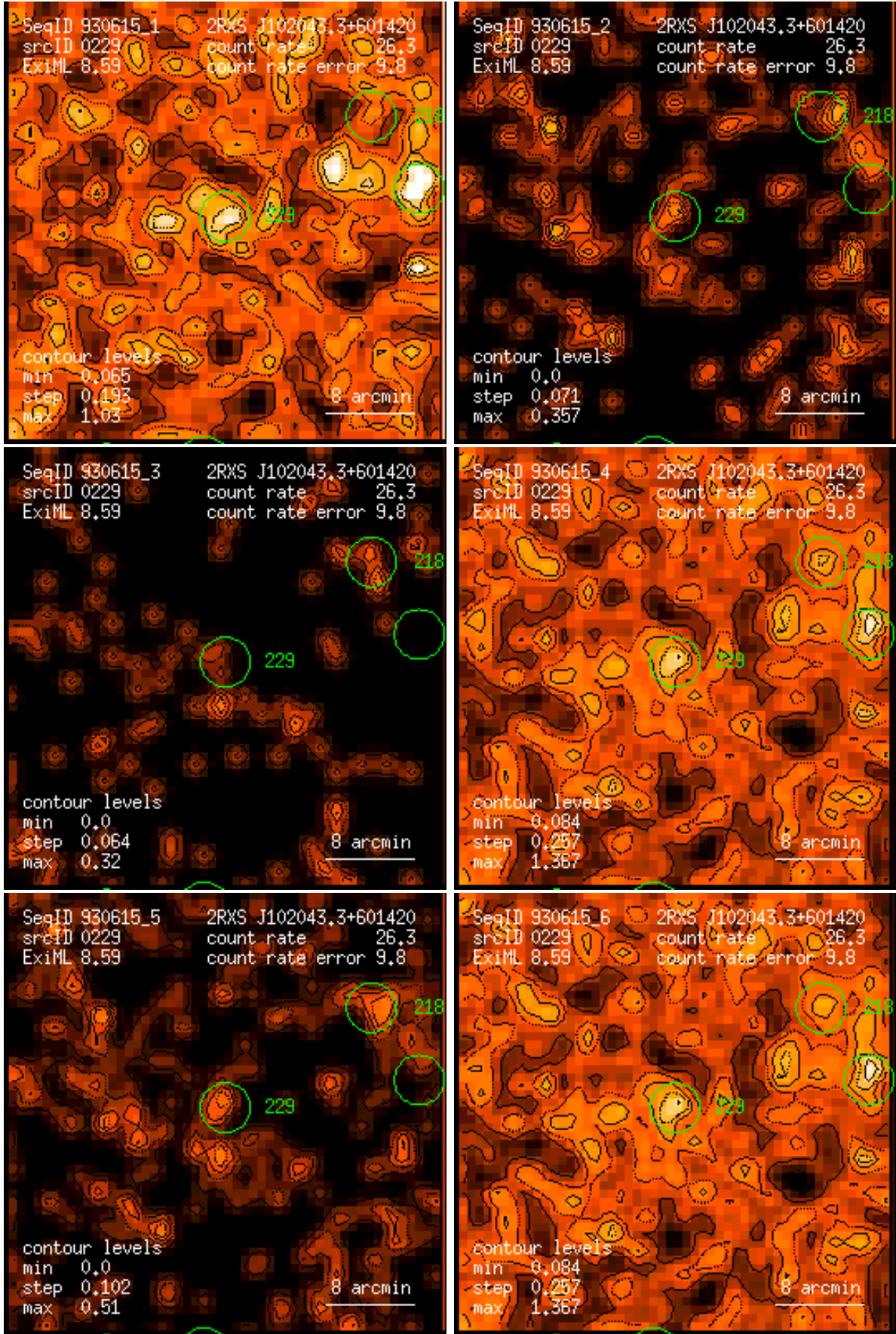
Figure 229: RASS 930615: detection 0229: band rate images, Gaussian filter: (1) PSPC channels 11 – 41, (2) 52 – 90, (3) 91 – 201, (4) 11 – 235, (5) 52 – 201, (6) 11 – 201. Broad band rates in counts/ks. Band rate contour levels in counts/ks/arcmin 2 .
