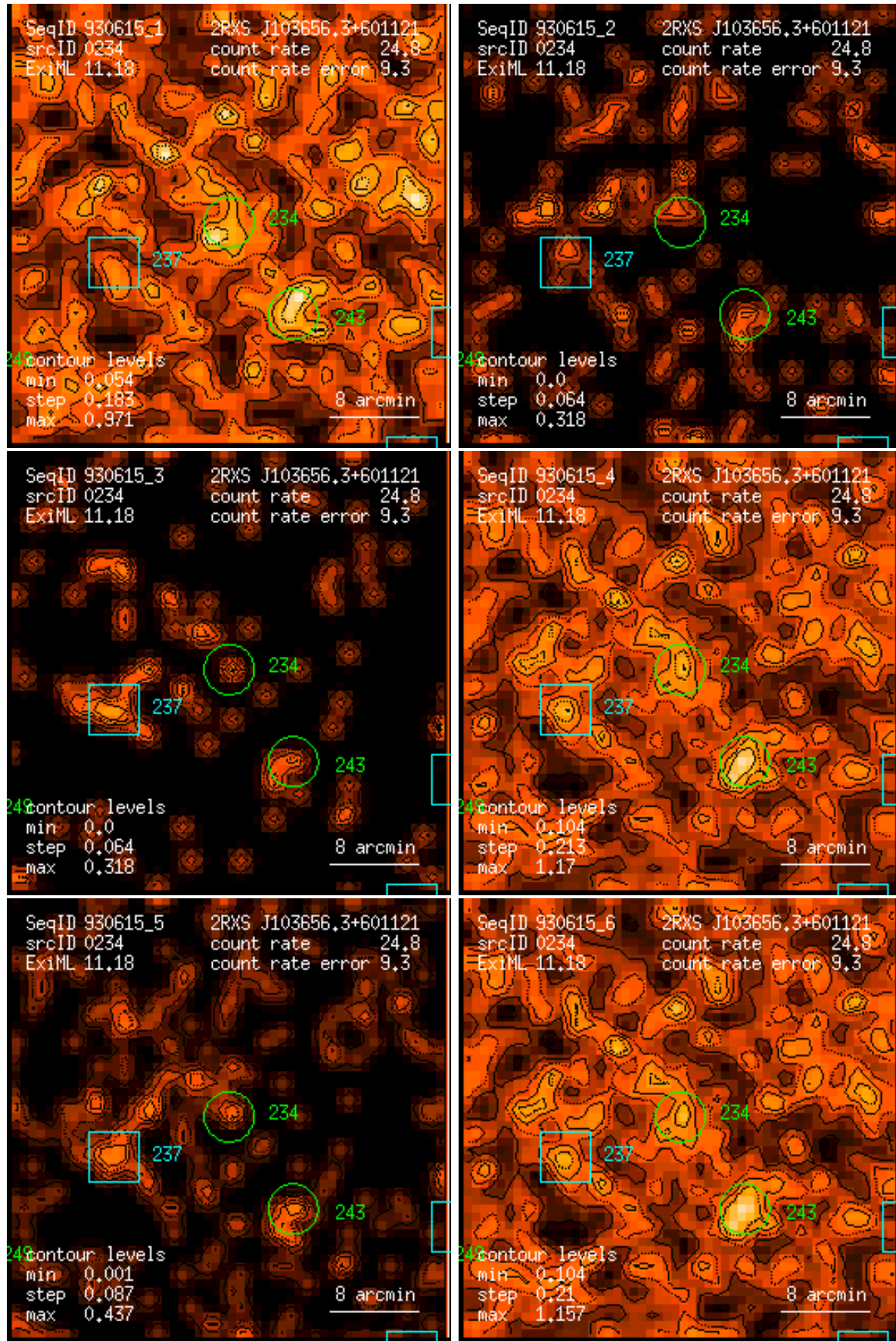
Figure 234: RASS 930615: detection 0234: band rate images, Gaussian filter: (1) PSPC channels 11 – 41, (2) 52 – 90, (3) 91 – 201, (4) 11 – 235, (5) 52 – 201, (6) 11 – 201. Broad band rates in counts/ks. Band rate contour levels in counts/ks/arcmin 2 .
