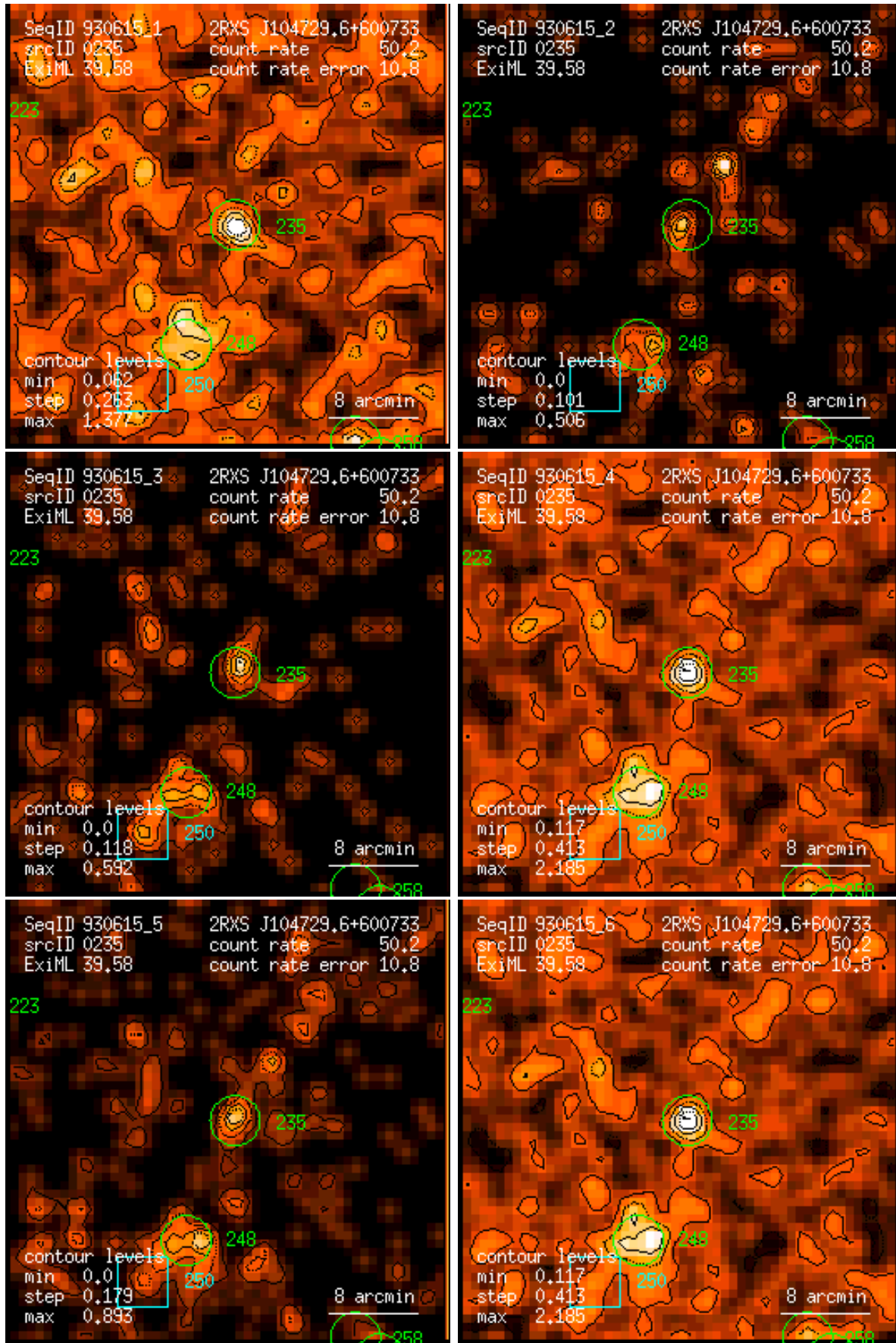
Figure 235: RASS 930615: detection 0235: band rate images, Gaussian filter: (1) PSPC channels 11 – 41, (2) 52 – 90, (3) 91 – 201, (4) 11 – 235, (5) 52 – 201, (6) 11 – 201. Broad band rates in counts/ks. Band rate contour levels in counts/ks/arcmin 2 .
