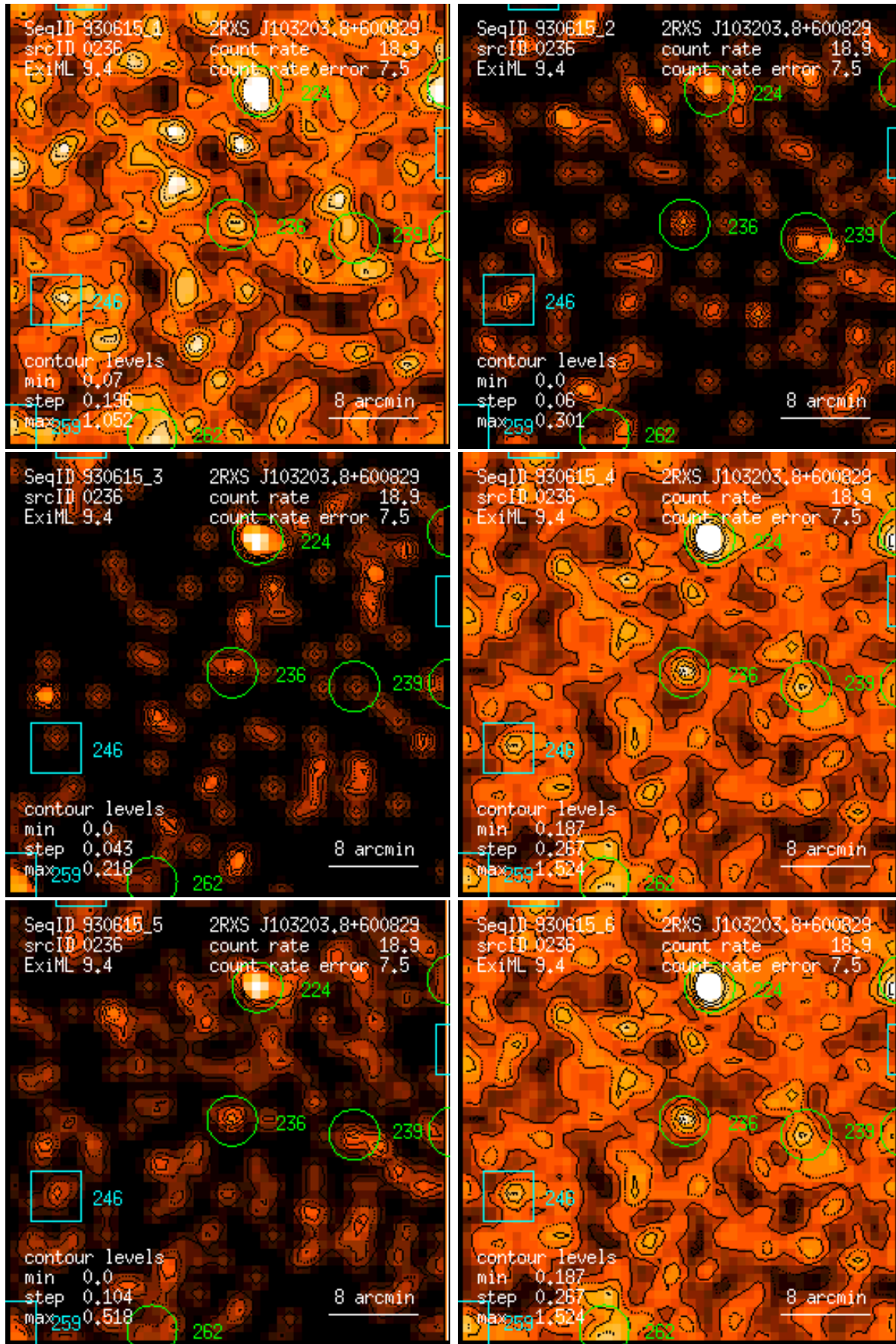
Figure 236: RASS 930615: detection 0236: band rate images, Gaussian filter: (1) PSPC channels 11 – 41, (2) 52 – 90, (3) 91 – 201, (4) 11 – 235, (5) 52 – 201, (6) 11 – 201. Broad band rates in counts/ks. Band rate contour levels in counts/ks/arcmin 2 .
