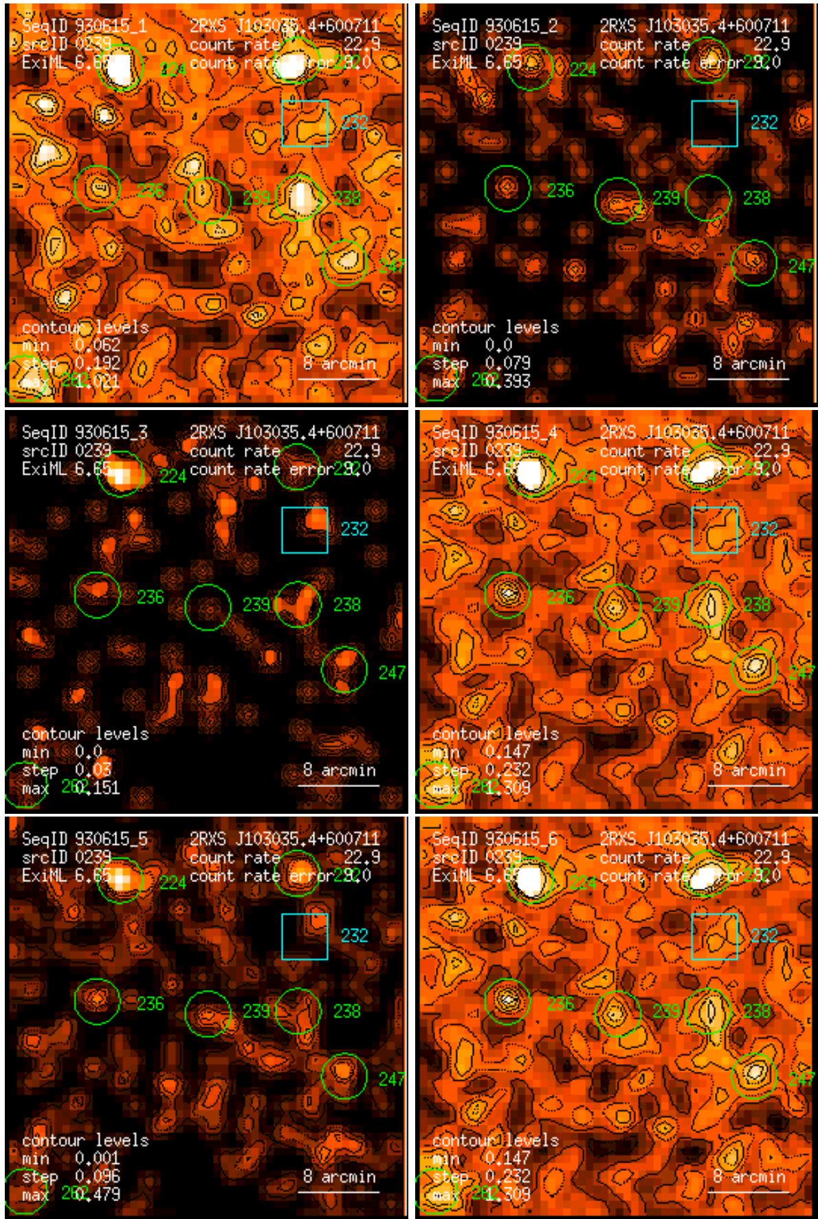
Figure 239: RASS 930615: detection 0239: band rate images, Gaussian filter: (1) PSPC channels 11 – 41, (2) 52 – 90, (3) 91 – 201, (4) 11 – 235, (5) 52 – 201, (6) 11 – 201. Broad band rates in counts/ks. Band rate contour levels in counts/ks/arcmin 2 .
