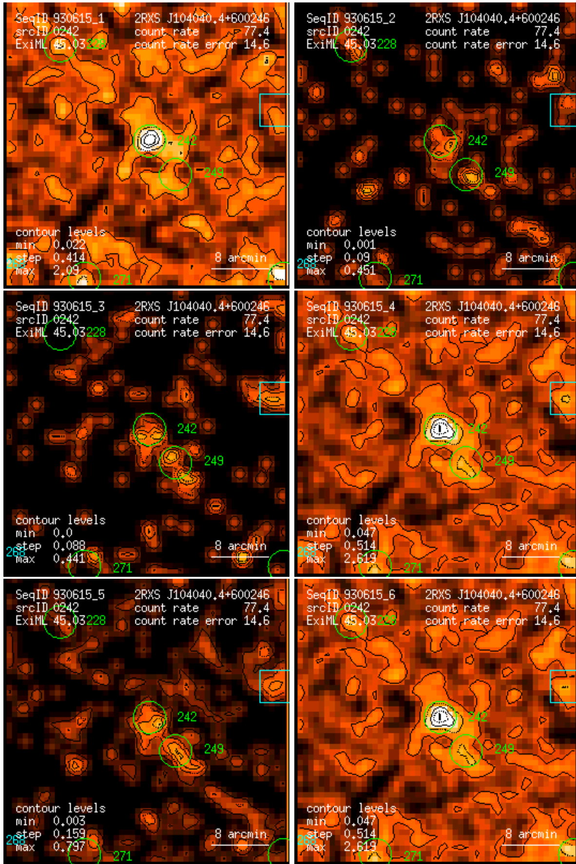
Figure 242: RASS 930615: detection 0242: band rate images, Gaussian filter: (1) PSPC channels 11 – 41, (2) 52 – 90, (3) 91 – 201, (4) 11 – 235, (5) 52 – 201, (6) 11 – 201. Broad band rates in counts/ks. Band rate contour levels in counts/ks/arcmin 2 .
