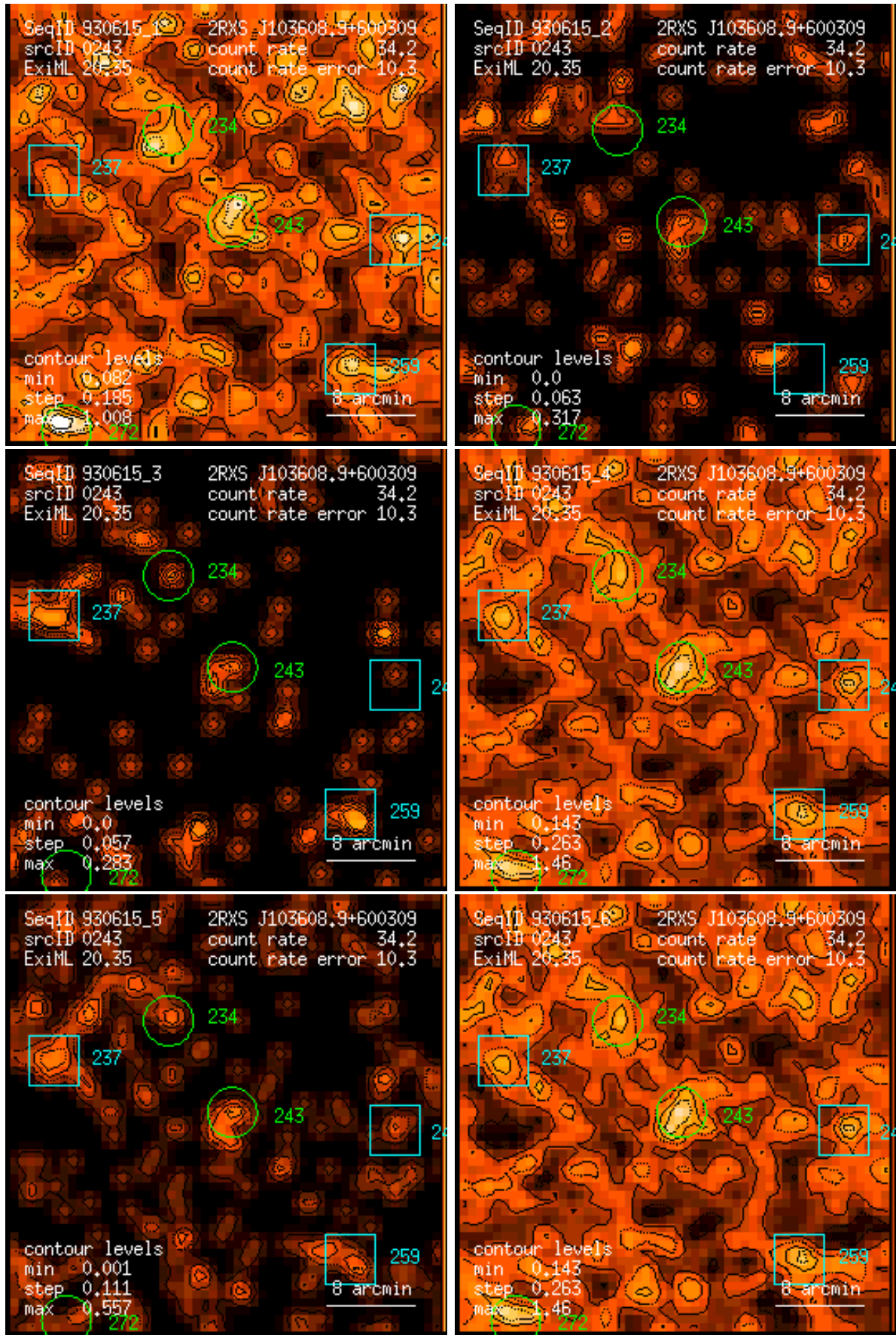
Figure 243: RASS 930615: detection 0243: band rate images, Gaussian filter: (1) PSPC channels 11 – 41, (2) 52 – 90, (3) 91 – 201, (4) 11 – 235, (5) 52 – 201, (6) 11 – 201. Broad band rates in counts/ks. Band rate contour levels in counts/ks/arcmin 2 .
