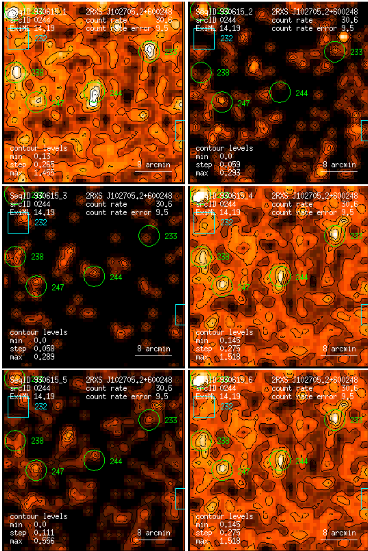
Figure 244: RASS 930615: detection 0244: band rate images, Gaussian filter: (1) PSPC channels 11 – 41, (2) 52 – 90, (3) 91 – 201, (4) 11 – 235, (5) 52 – 201, (6) 11 – 201. Broad band rates in counts/ks. Band rate contour levels in counts/ks/arcmin 2 .
