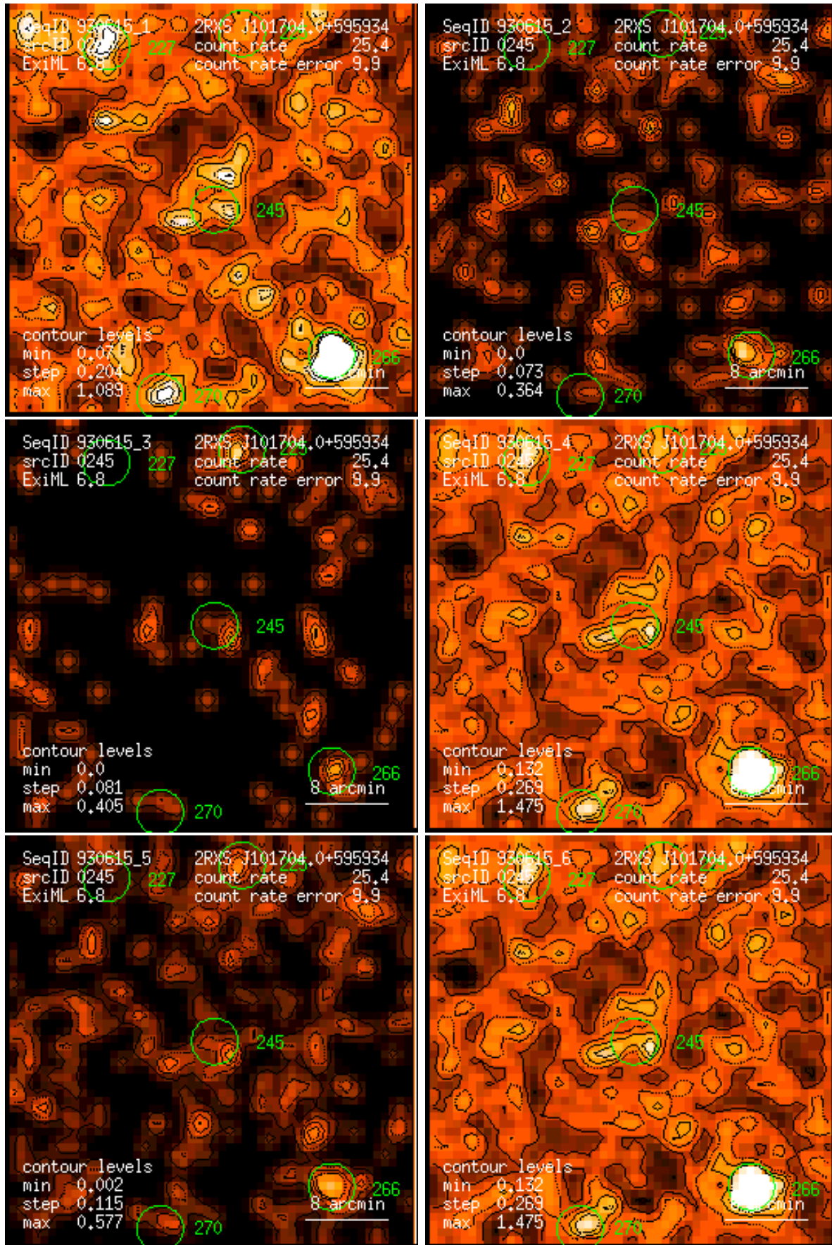
Figure 245: RASS 930615: detection 0245: band rate images, Gaussian filter: (1) PSPC channels 11 – 41, (2) 52 – 90, (3) 91 – 201, (4) 11 – 235, (5) 52 – 201, (6) 11 – 201. Broad band rates in counts/ks. Band rate contour levels in counts/ks/arcmin 2 .
