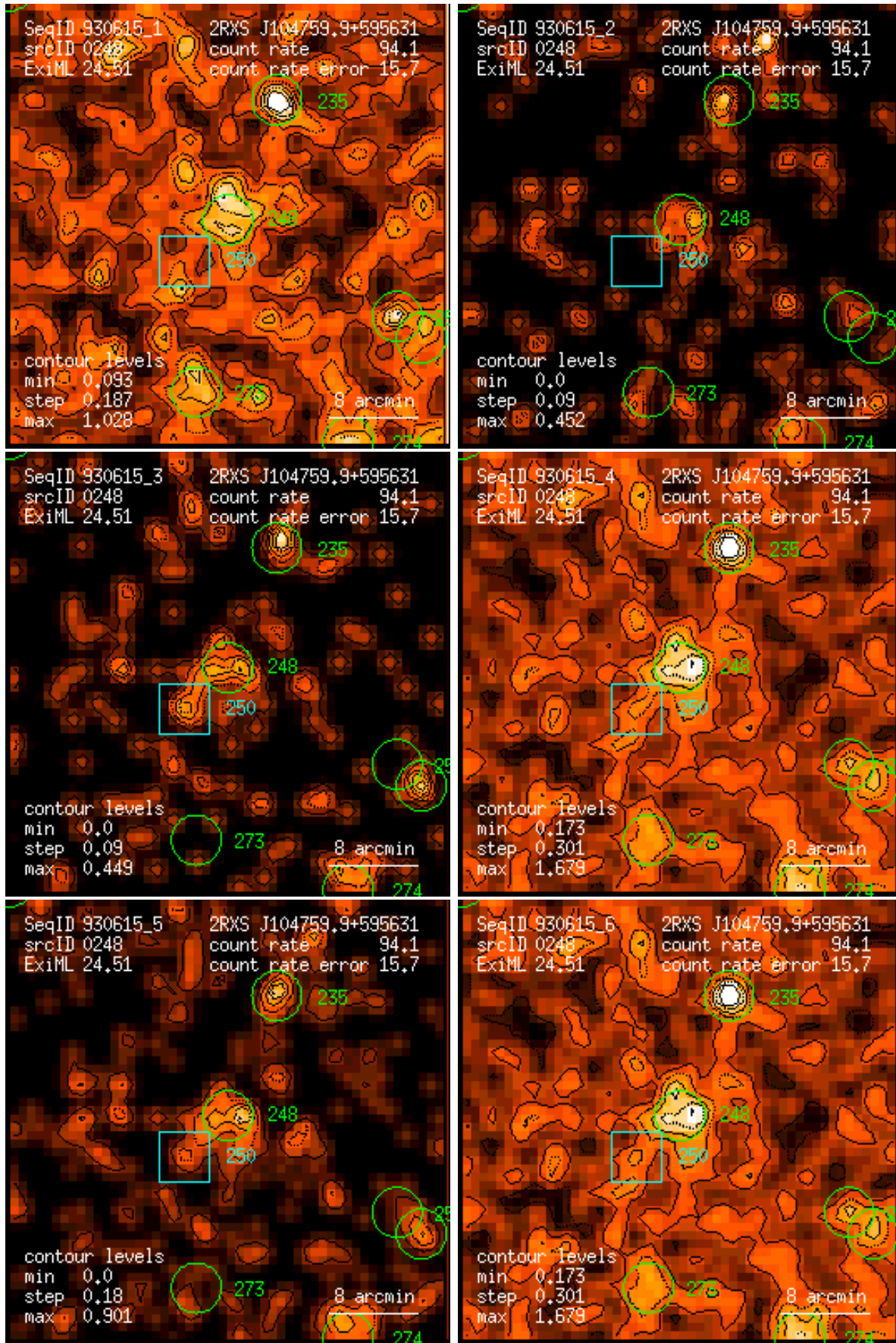
Figure 248: RASS 930615: detection 0248: band rate images, Gaussian filter: (1) PSPC channels 11 – 41, (2) 52 – 90, (3) 91 – 201, (4) 11 – 235, (5) 52 – 201, (6) 11 – 201. Broad band rates in counts/ks. Band rate contour levels in counts/ks/arcmin 2 .
