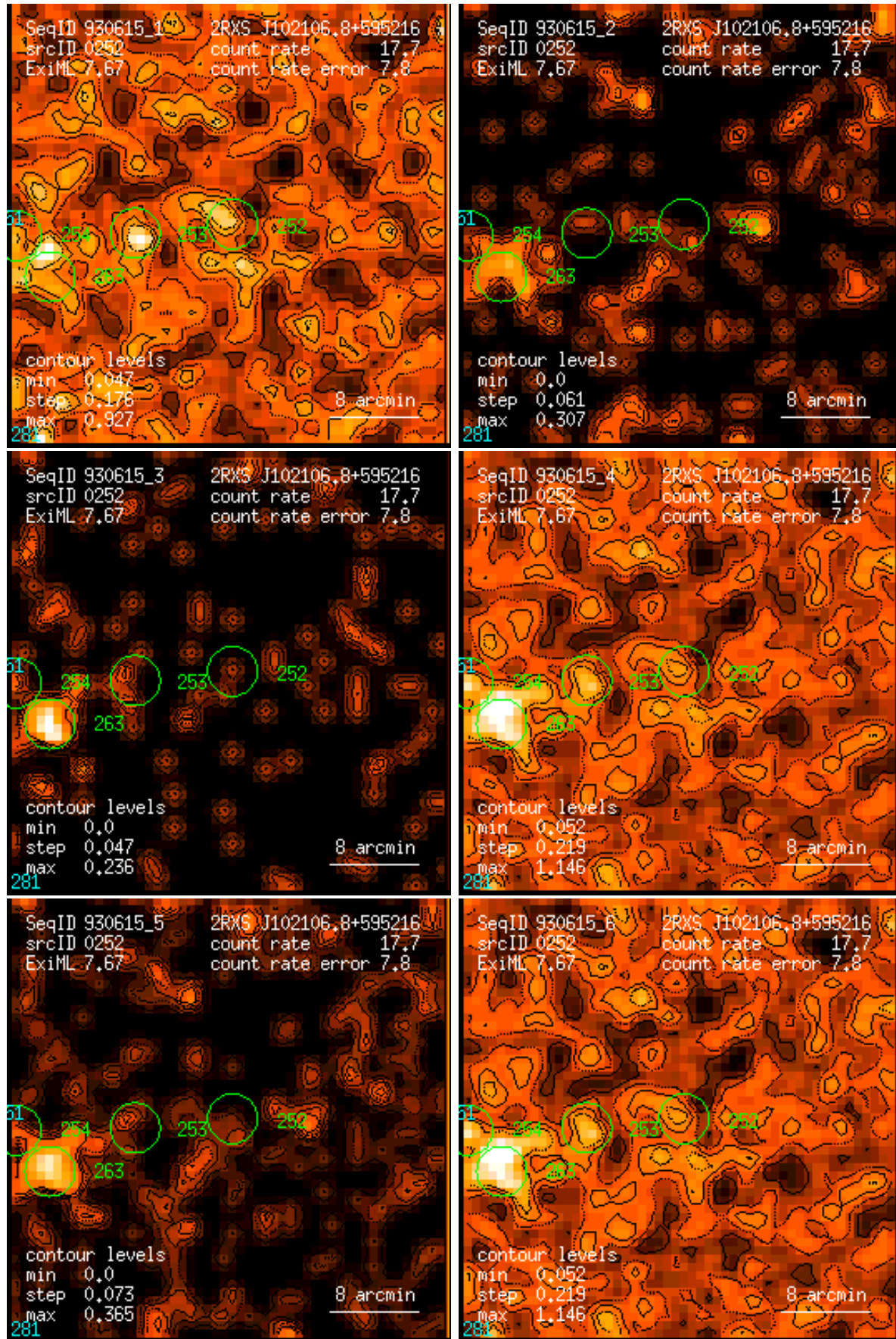
Figure 252: RASS 930615: detection 0252: band rate images, Gaussian filter: (1) PSPC channels 11 – 41, (2) 52 – 90, (3) 91 – 201, (4) 11 – 235, (5) 52 – 201, (6) 11 – 201. Broad band rates in counts/ks. Band rate contour levels in counts/ks/arcmin 2 .
