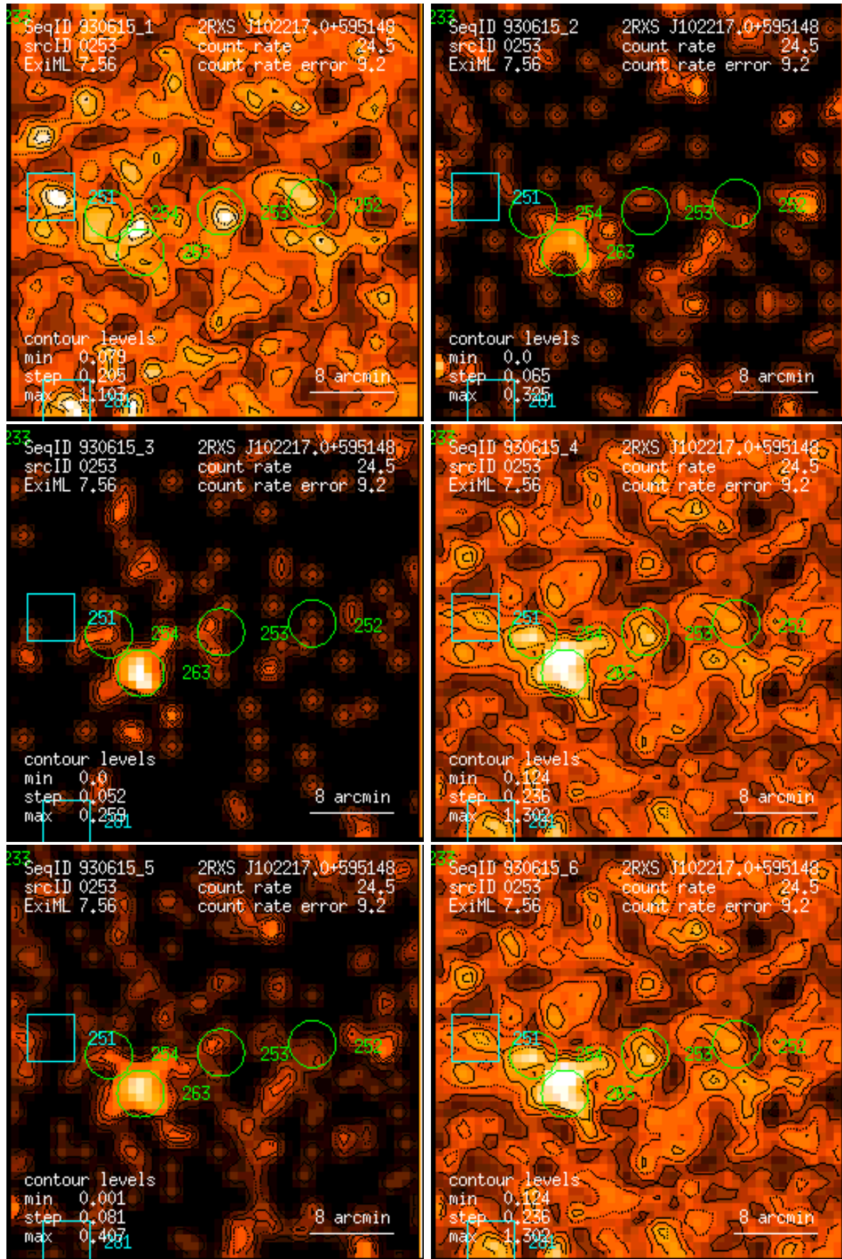
Figure 253: RASS 930615: detection 0253: band rate images, Gaussian filter: (1) PSPC channels 11 – 41, (2) 52 – 90, (3) 91 – 201, (4) 11 – 235, (5) 52 – 201, (6) 11 – 201. Broad band rates in counts/ks. Band rate contour levels in counts/ks/arcmin 2 .
