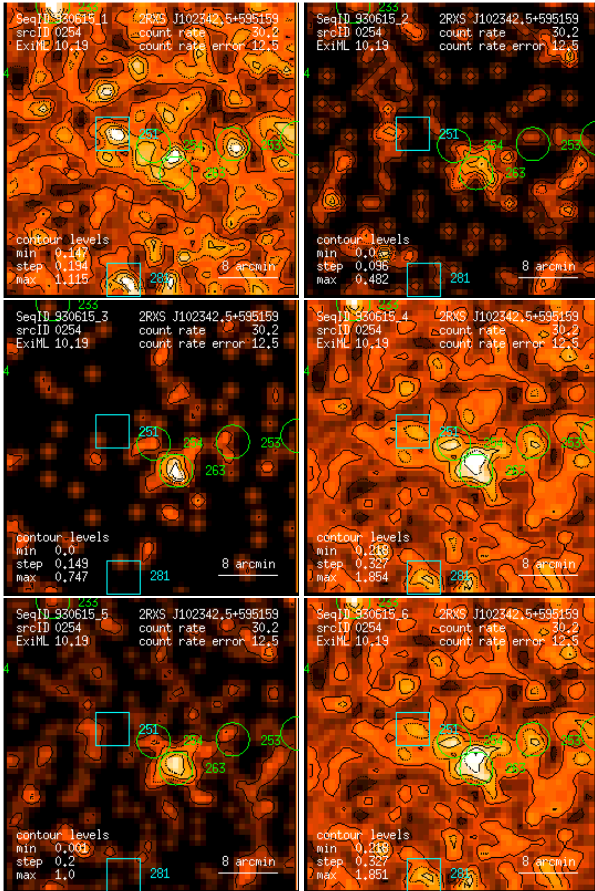
Figure 254: RASS 930615: detection 0254: band rate images, Gaussian filter: (1) PSPC channels 11 – 41, (2) 52 – 90, (3) 91 – 201, (4) 11 – 235, (5) 52 – 201, (6) 11 – 201. Broad band rates in counts/ks. Band rate contour levels in counts/ks/arcmin 2 .
