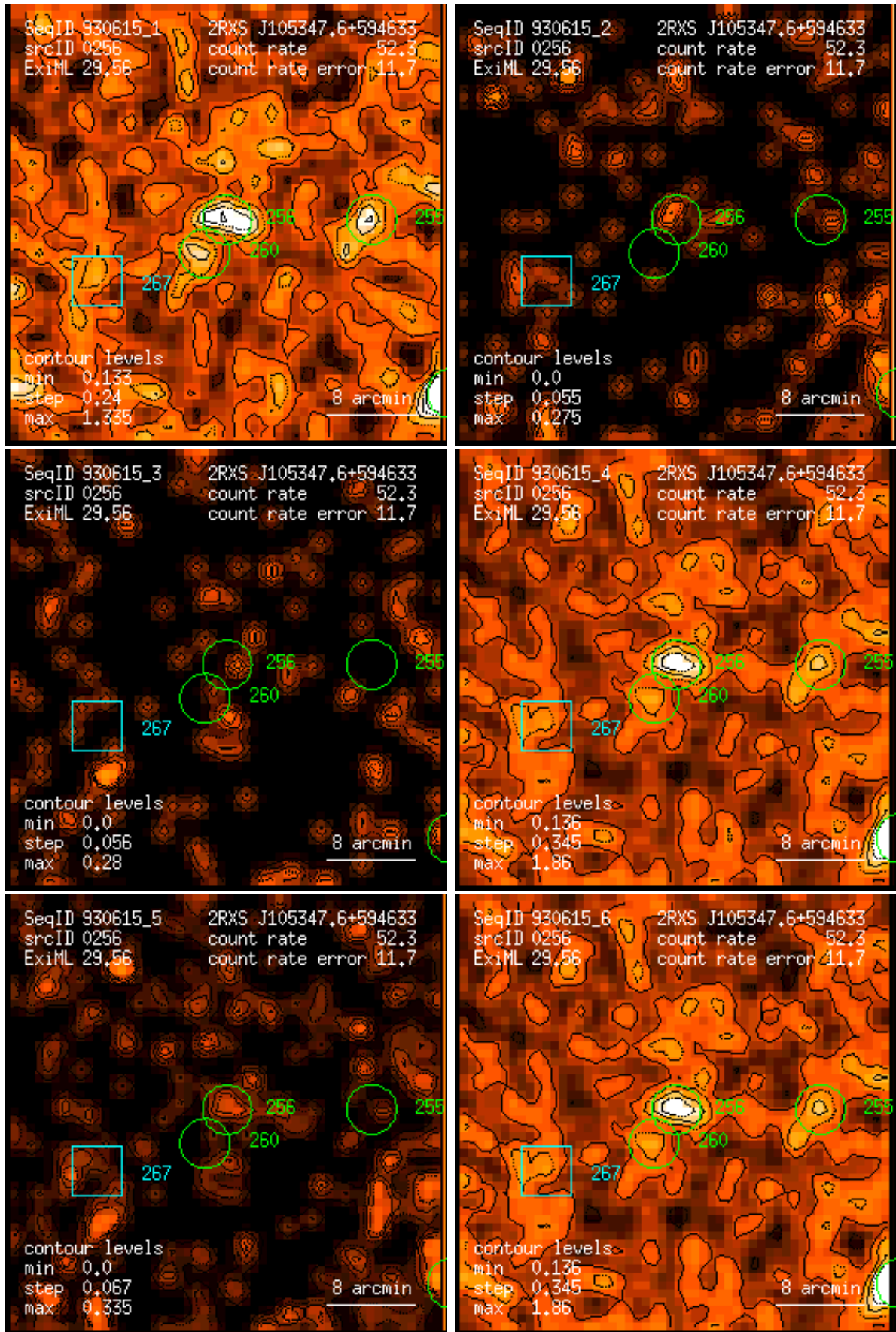
Figure 256: RASS 930615: detection 0256: band rate images, Gaussian filter: (1) PSPC channels 11 – 41, (2) 52 – 90, (3) 91 – 201, (4) 11 – 235, (5) 52 – 201, (6) 11 – 201. Broad band rates in counts/ks. Band rate contour levels in counts/ks/arcmin 2 .
