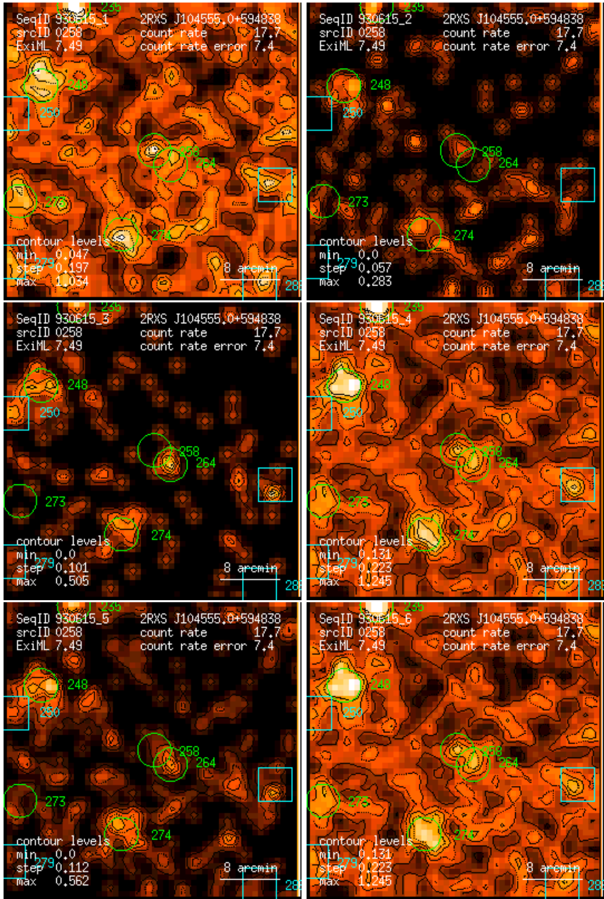
Figure 258: RASS 930615: detection 0258: band rate images, Gaussian filter: (1) PSPC channels 11 – 41, (2) 52 – 90, (3) 91 – 201, (4) 11 – 235, (5) 52 – 201, (6) 11 – 201. Broad band rates in counts/ks. Band rate contour levels in counts/ks/arcmin 2 .
