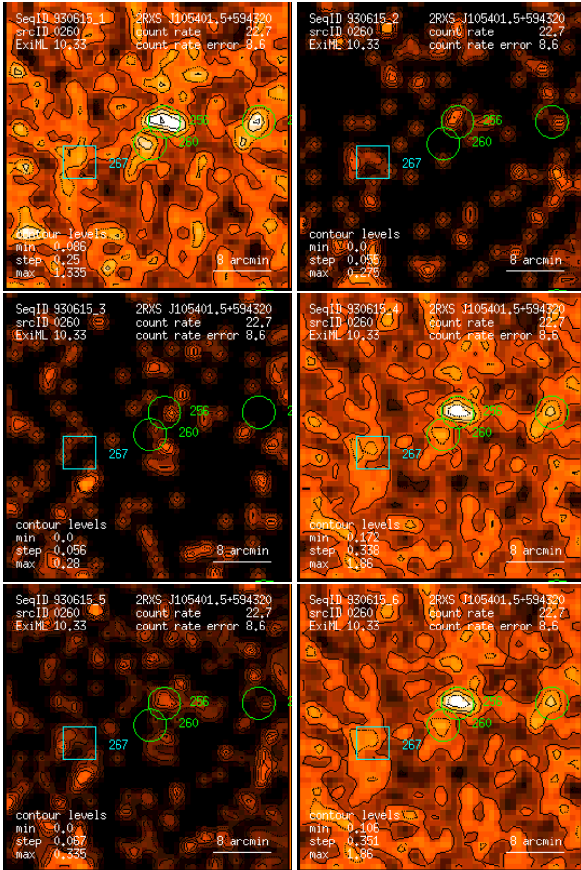
Figure 260: RASS 930615: detection 0260: band rate images, Gaussian filter: (1) PSPC channels 11 – 41, (2) 52 – 90, (3) 91 – 201, (4) 11 – 235, (5) 52 – 201, (6) 11 – 201. Broad band rates in counts/ks. Band rate contour levels in counts/ks/arcmin 2 .
