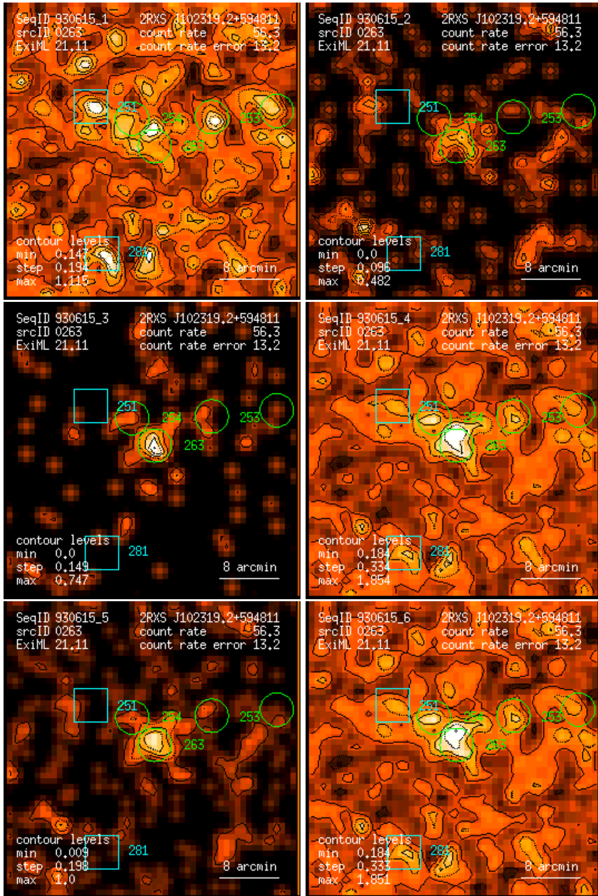
Figure 263: RASS 930615: detection 0263: band rate images, Gaussian filter: (1) PSPC channels 11 – 41, (2) 52 – 90, (3) 91 – 201, (4) 11 – 235, (5) 52 – 201, (6) 11 – 201. Broad band rates in counts/ks. Band rate contour levels in counts/ks/arcmin 2 .
