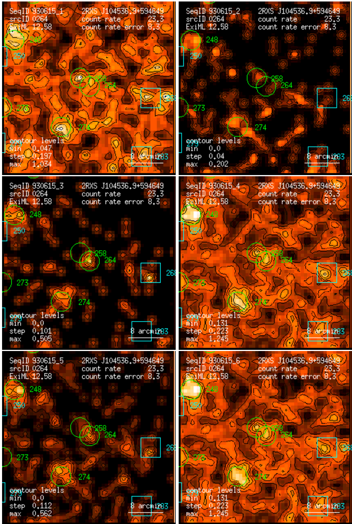
Figure 264: RASS 930615: detection 0264: band rate images, Gaussian filter: (1) PSPC channels 11 – 41, (2) 52 – 90, (3) 91 – 201, (4) 11 – 235, (5) 52 – 201, (6) 11 – 201. Broad band rates in counts/ks. Band rate contour levels in counts/ks/arcmin 2 .
