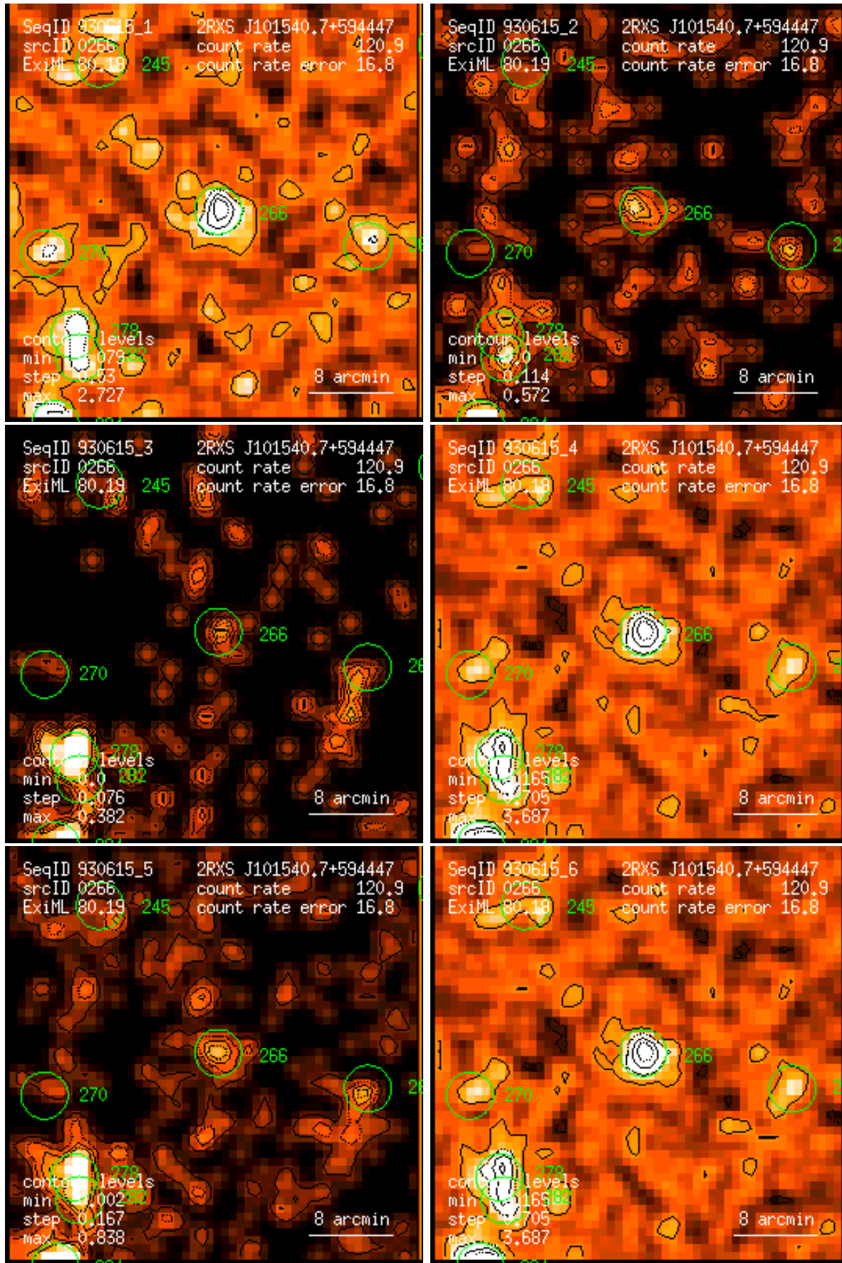
Figure 266: RASS 930615: detection 0266: band rate images, Gaussian filter: (1) PSPC channels 11 – 41, (2) 52 – 90, (3) 91 – 201, (4) 11 – 235, (5) 52 – 201, (6) 11 – 201. Broad band rates in counts/ks. Band rate contour levels in counts/ks/arcmin 2 .
