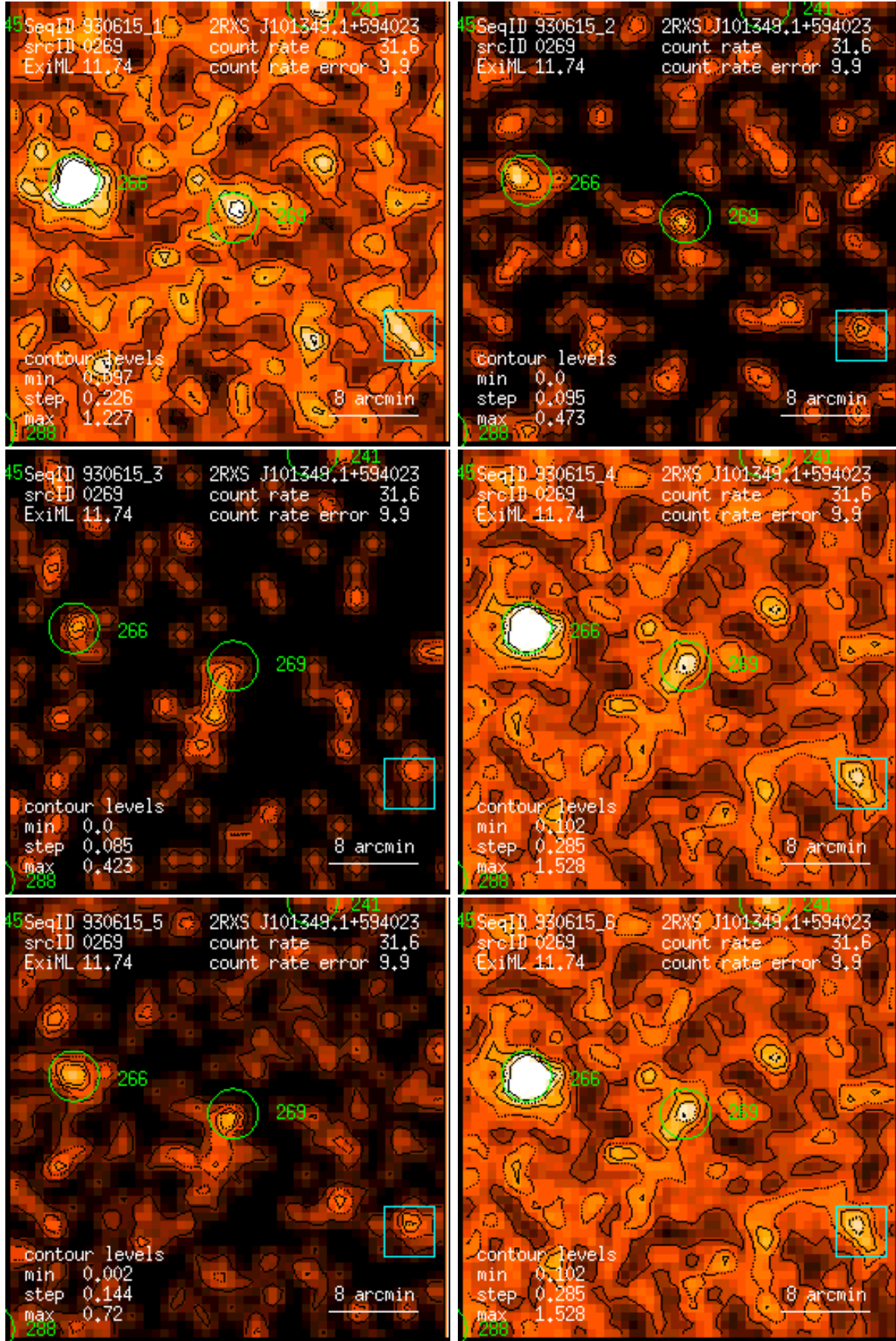
Figure 269: RASS 930615: detection 0269: band rate images, Gaussian filter: (1) PSPC channels 11 – 41, (2) 52 – 90, (3) 91 – 201, (4) 11 – 235, (5) 52 – 201, (6) 11 – 201. Broad band rates in counts/ks. Band rate contour levels in counts/ks/arcmin 2 .
