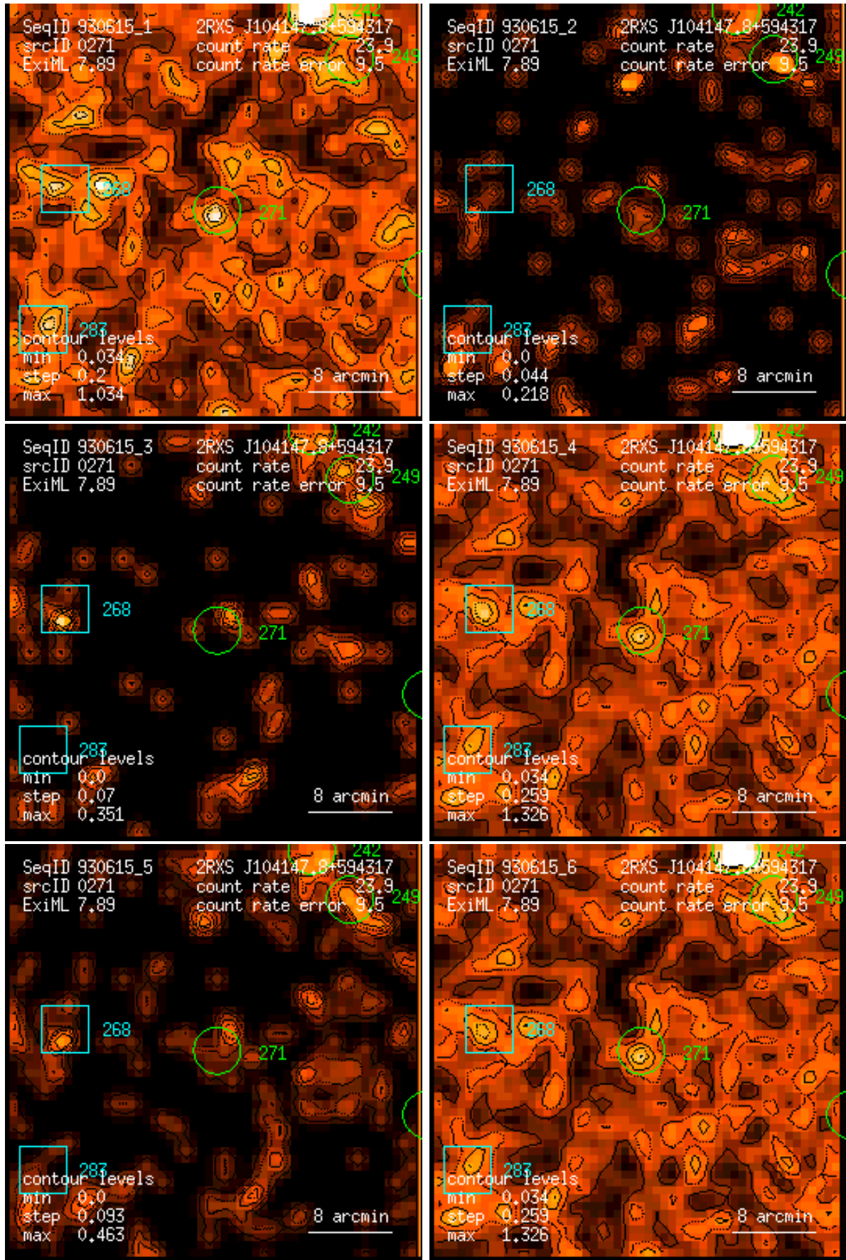
Figure 271: RASS 930615: detection 0271: band rate images, Gaussian filter: (1) PSPC channels 11 – 41, (2) 52 – 90, (3) 91 – 201, (4) 11 – 235, (5) 52 – 201, (6) 11 – 201. Broad band rates in counts/ks. Band rate contour levels in counts/ks/arcmin 2 .
