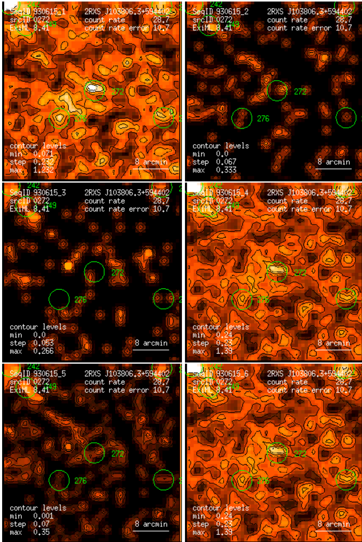
Figure 272: RASS 930615: detection 0272: band rate images, Gaussian filter: (1) PSPC channels 11 – 41, (2) 52 – 90, (3) 91 – 201, (4) 11 – 235, (5) 52 – 201, (6) 11 – 201. Broad band rates in counts/ks. Band rate contour levels in counts/ks/arcmin 2 .
