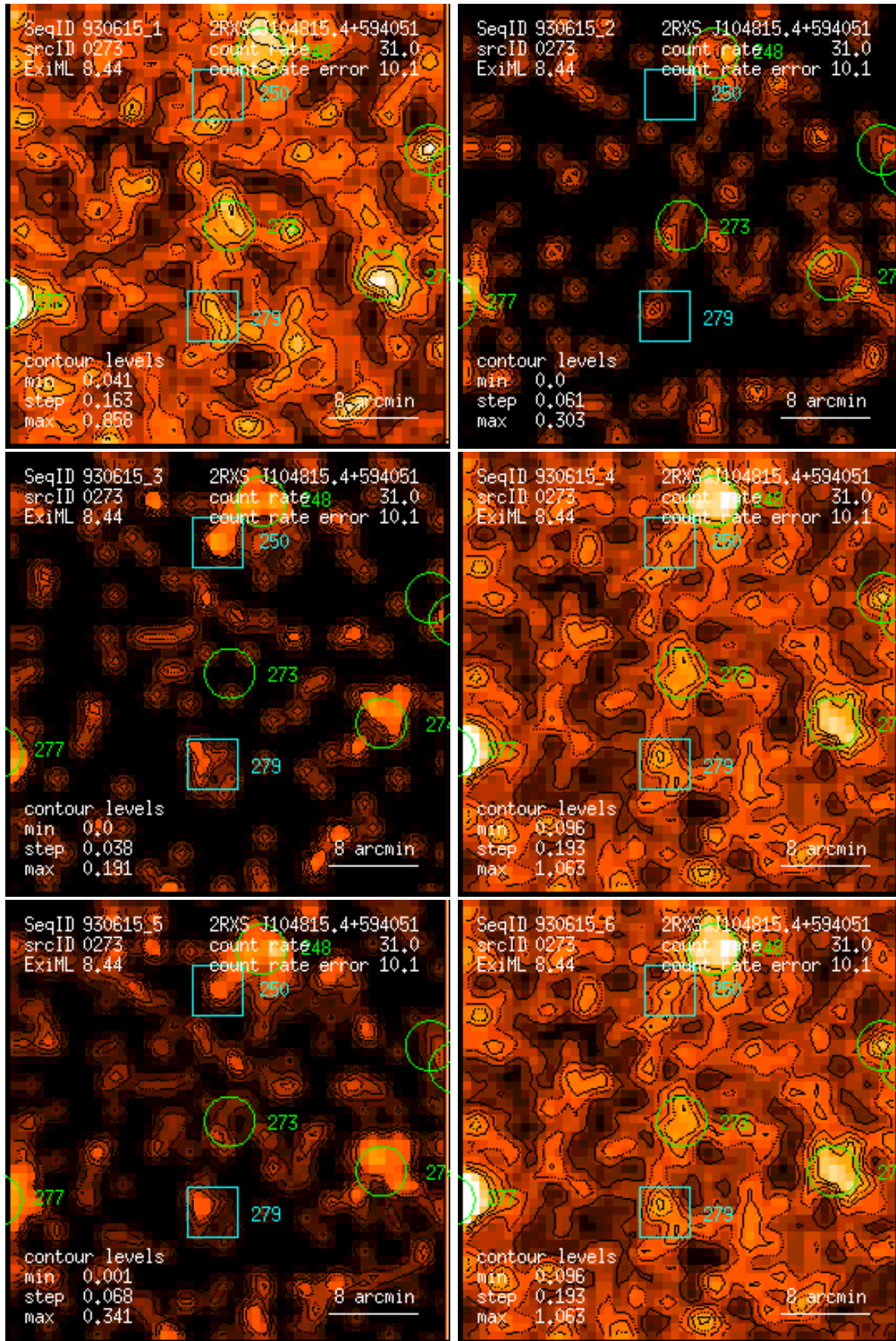
Figure 273: RASS 930615: detection 0273: band rate images, Gaussian filter: (1) PSPC channels 11 – 41, (2) 52 – 90, (3) 91 – 201, (4) 11 – 235, (5) 52 – 201, (6) 11 – 201. Broad band rates in counts/ks. Band rate contour levels in counts/ks/arcmin 2 .
