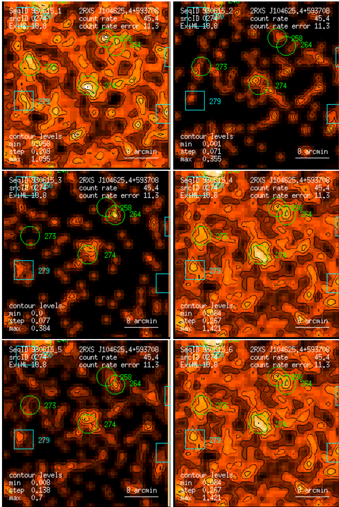
Figure 274: RASS 930615: detection 0274: band rate images, Gaussian filter: (1) PSPC channels 11 – 41, (2) 52 – 90, (3) 91 – 201, (4) 11 – 235, (5) 52 – 201, (6) 11 – 201. Broad band rates in counts/ks. Band rate contour levels in counts/ks/arcmin 2 .
