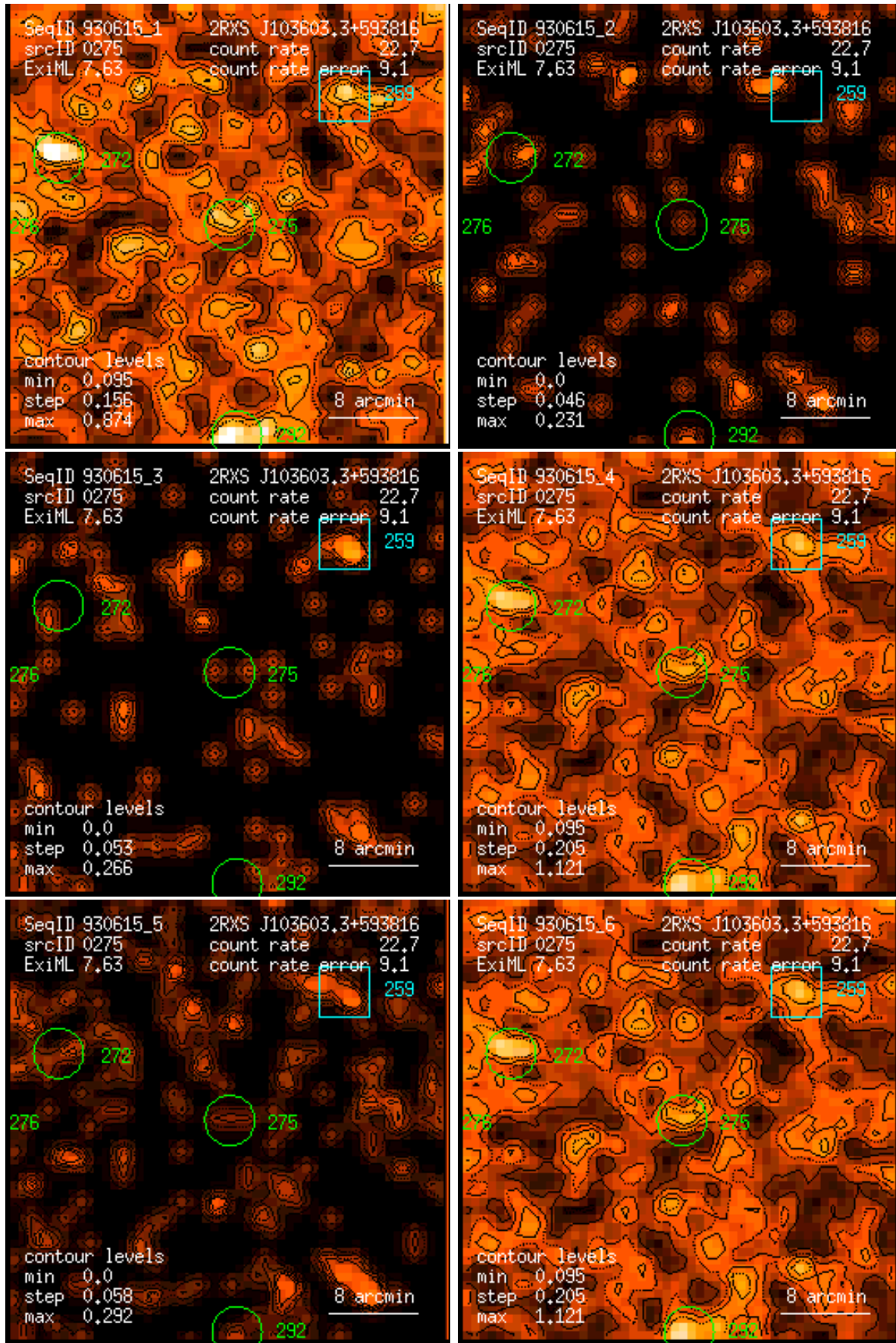
Figure 275: RASS 930615: detection 0275: band rate images, Gaussian filter: (1) PSPC channels 11 – 41, (2) 52 – 90, (3) 91 – 201, (4) 11 – 235, (5) 52 – 201, (6) 11 – 201. Broad band rates in counts/ks. Band rate contour levels in counts/ks/arcmin 2 .
