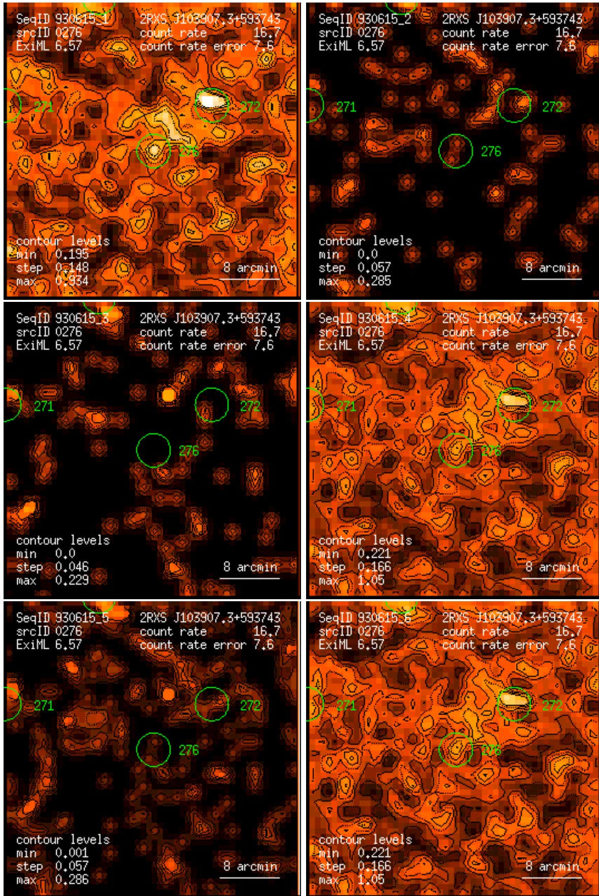
Figure 276: RASS 930615: detection 0276: band rate images, Gaussian filter: (1) PSPC channels 11 – 41, (2) 52 – 90, (3) 91 – 201, (4) 11 – 235, (5) 52 – 201, (6) 11 – 201. Broad band rates in counts/ks. Band rate contour levels in counts/ks/arcmin 2 .
