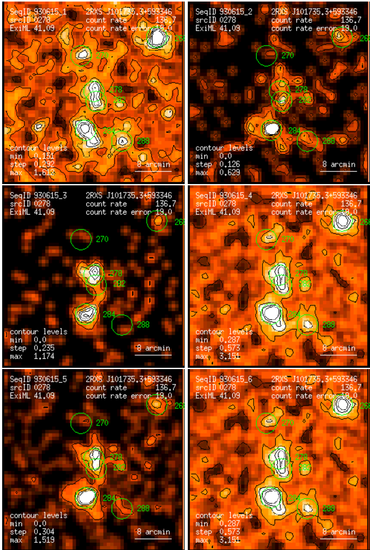
Figure 278: RASS 930615: detection 0278: band rate images, Gaussian filter: (1) PSPC channels 11 – 41, (2) 52 – 90, (3) 91 – 201, (4) 11 – 235, (5) 52 – 201, (6) 11 – 201. Broad band rates in counts/ks. Band rate contour levels in counts/ks/arcmin 2 .
