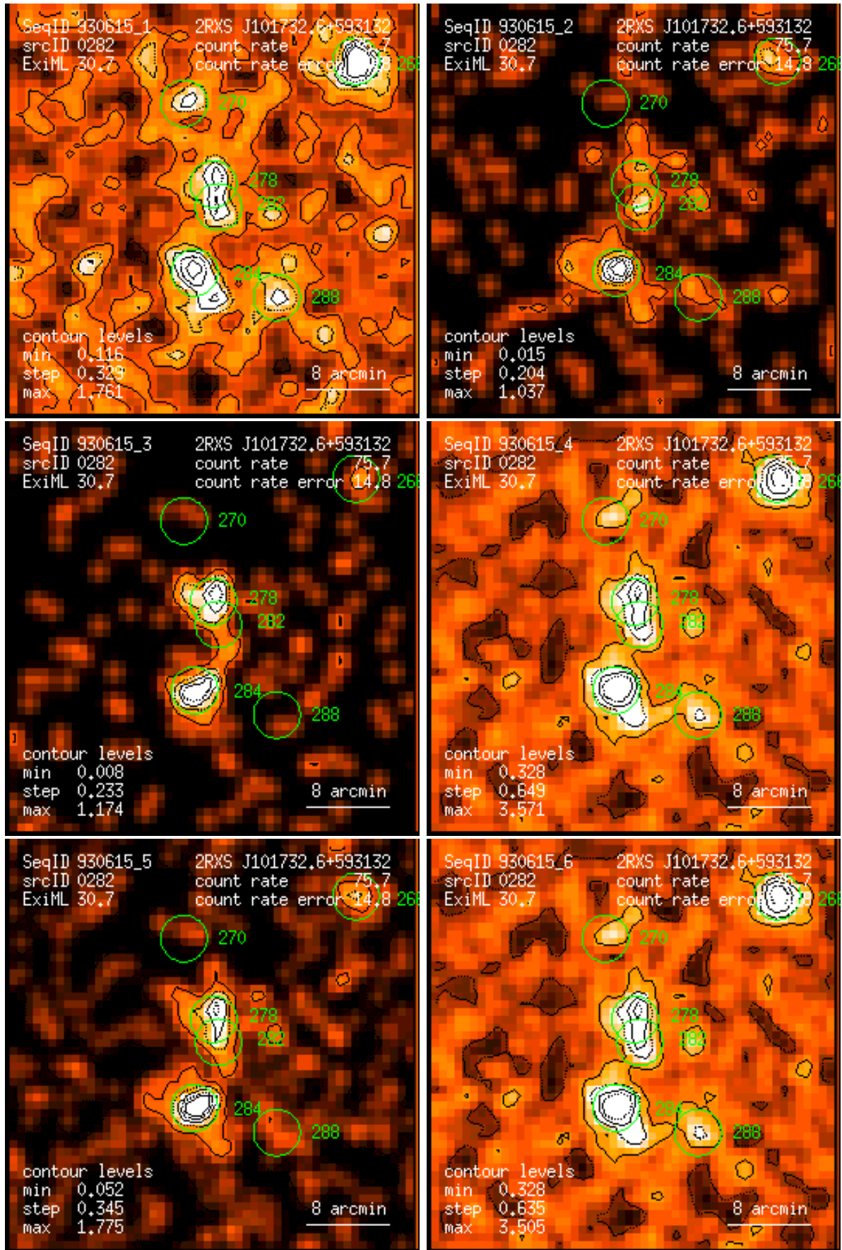
Figure 282: RASS 930615: detection 0282: band rate images, Gaussian filter: (1) PSPC channels 11 – 41, (2) 52 – 90, (3) 91 – 201, (4) 11 – 235, (5) 52 – 201, (6) 11 – 201. Broad band rates in counts/ks. Band rate contour levels in counts/ks/arcmin 2 .
