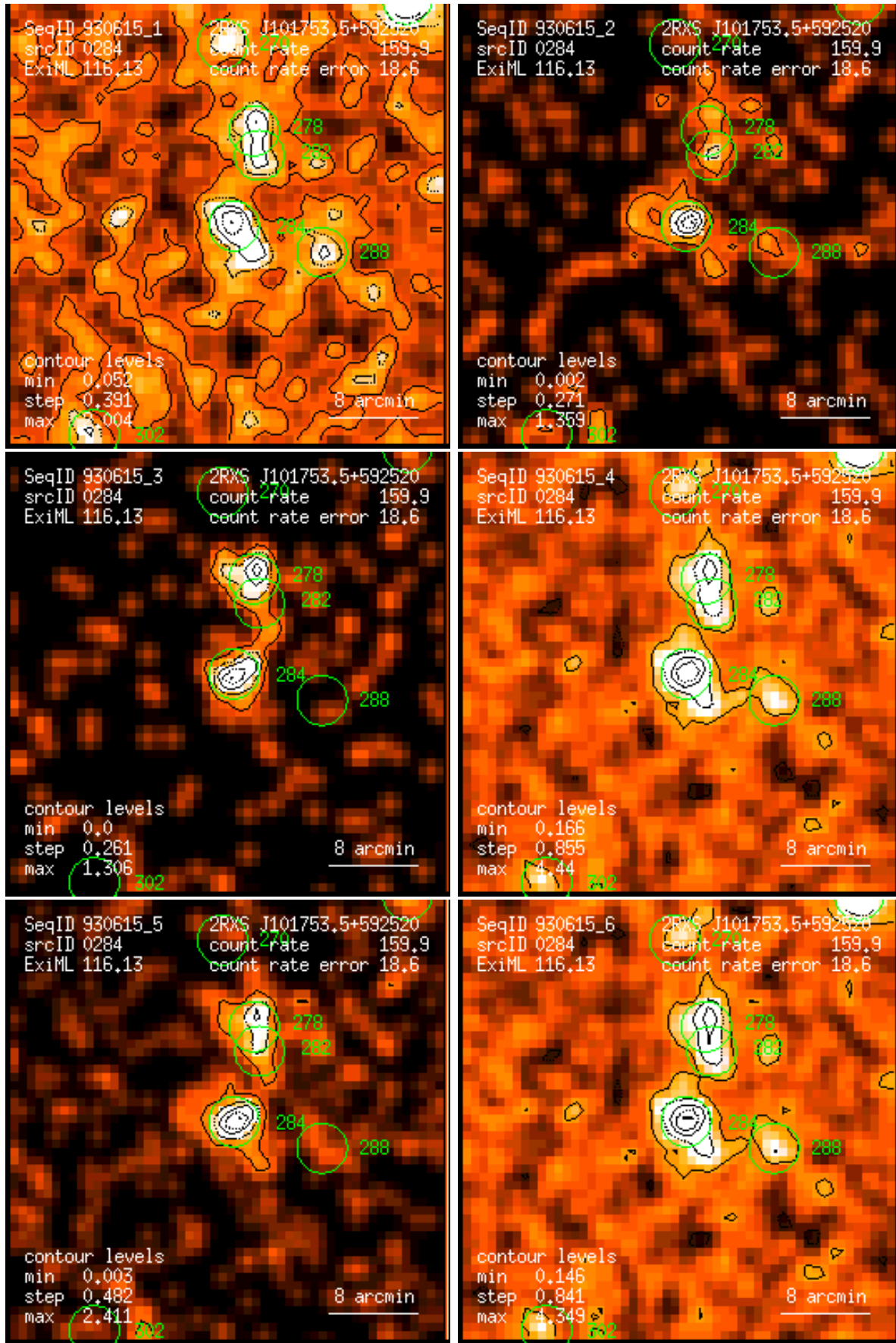
Figure 284: RASS 930615: detection 0284: band rate images, Gaussian filter: (1) PSPC channels 11 – 41, (2) 52 – 90, (3) 91 – 201, (4) 11 – 235, (5) 52 – 201, (6) 11 – 201. Broad band rates in counts/ks. Band rate contour levels in counts/ks/arcmin 2 .
