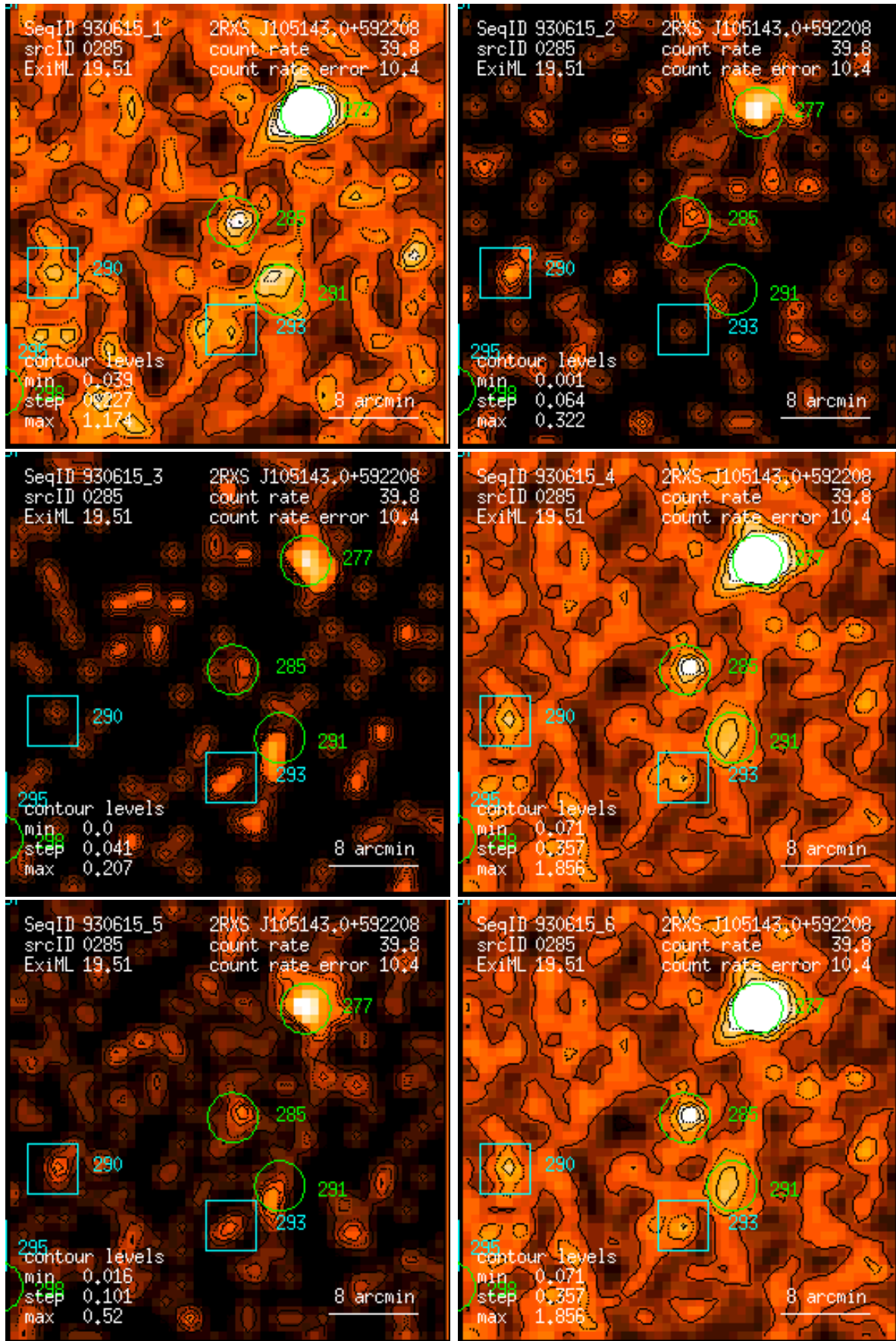
Figure 285: RASS 930615: detection 0285: band rate images, Gaussian filter: (1) PSPC channels 11 – 41, (2) 52 – 90, (3) 91 – 201, (4) 11 – 235, (5) 52 – 201, (6) 11 – 201. Broad band rates in counts/ks. Band rate contour levels in counts/ks/arcmin 2 .
