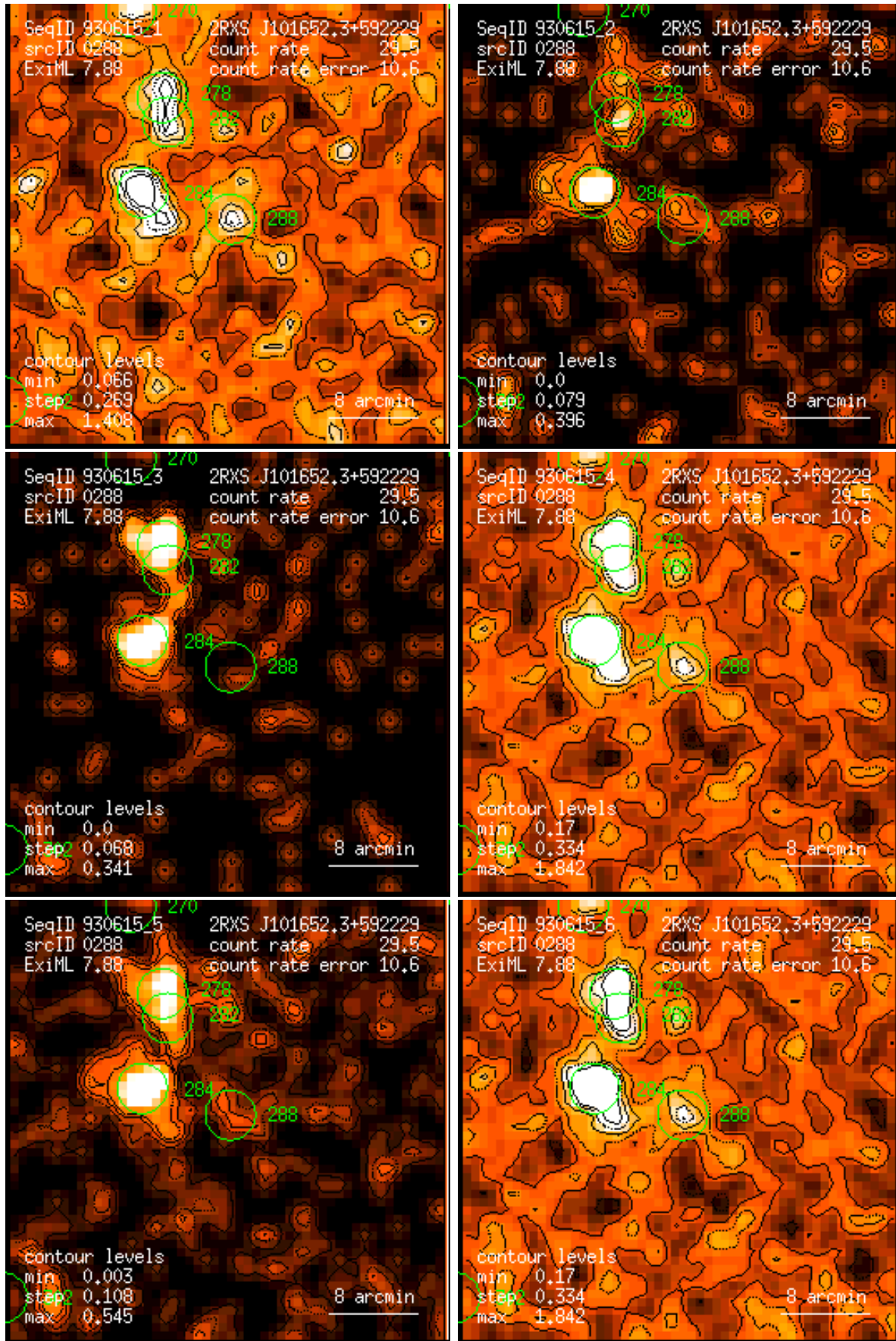
Figure 288: RASS 930615: detection 0288: band rate images, Gaussian filter: (1) PSPC channels 11 – 41, (2) 52 – 90, (3) 91 – 201, (4) 11 – 235, (5) 52 – 201, (6) 11 – 201. Broad band rates in counts/ks. Band rate contour levels in counts/ks/arcmin 2 .
