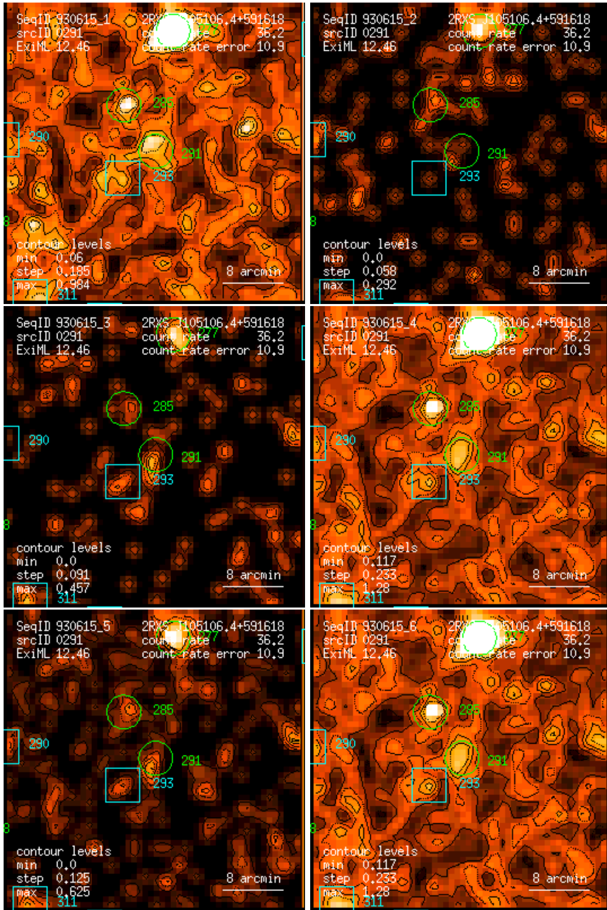
Figure 291: RASS 930615: detection 0291: band rate images, Gaussian filter: (1) PSPC channels 11 – 41, (2) 52 – 90, (3) 91 – 201, (4) 11 – 235, (5) 52 – 201, (6) 11 – 201. Broad band rates in counts/ks. Band rate contour levels in counts/ks/arcmin 2 .
