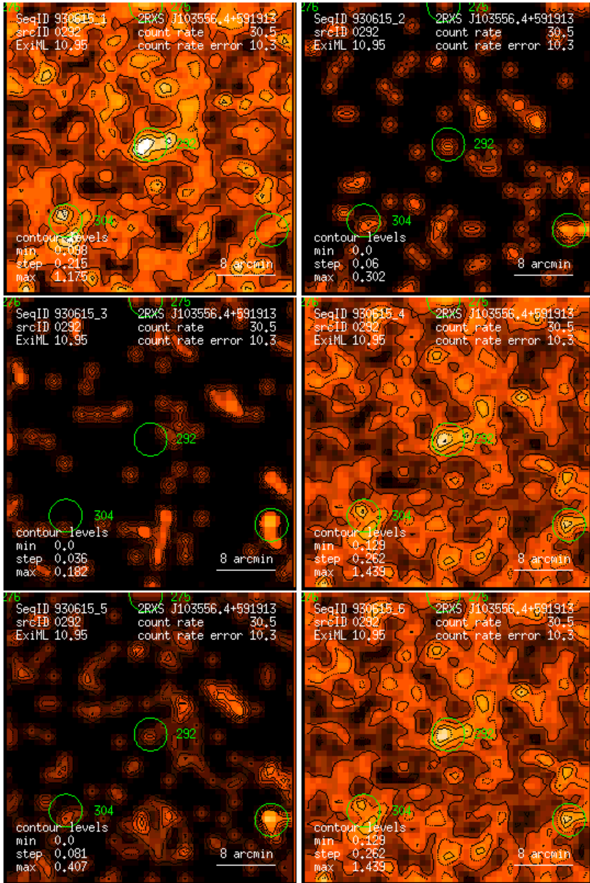
Figure 292: RASS 930615: detection 0292: band rate images, Gaussian filter: (1) PSPC channels 11 – 41, (2) 52 – 90, (3) 91 – 201, (4) 11 – 235, (5) 52 – 201, (6) 11 – 201. Broad band rates in counts/ks. Band rate contour levels in counts/ks/arcmin 2 .
